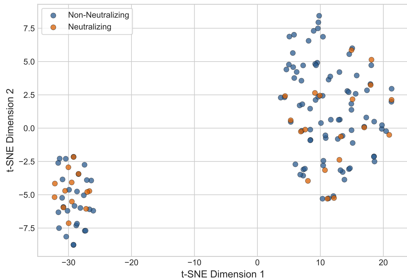
B. t-SNE Projection of Fused Feature Representations (Perplexity=30)
