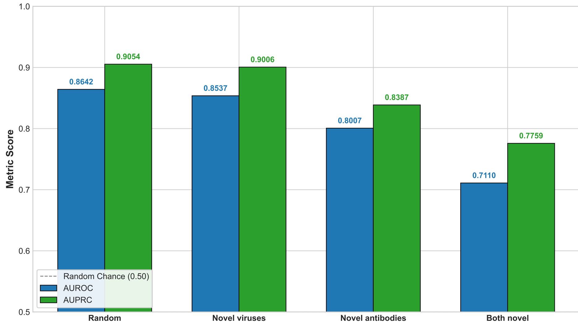
Figure 6.1: Logistic Regression Benchmark Performance Across Generalization Boundaries
