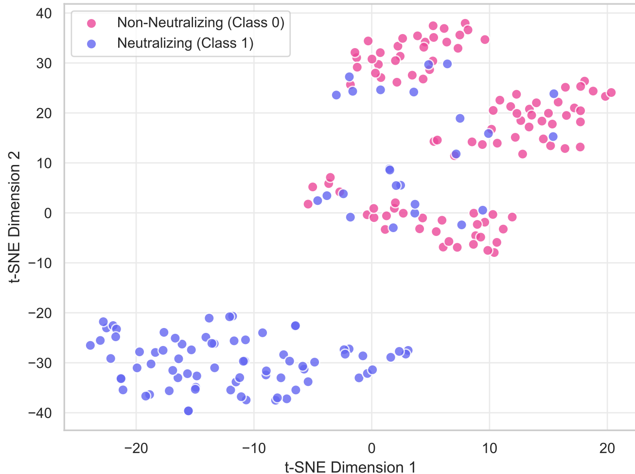
ESM-Mamba Fused Feature Space (t-SNE)
