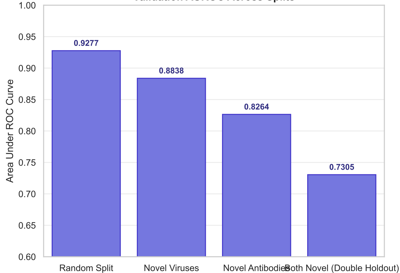
Validation AUROC Across Splits
