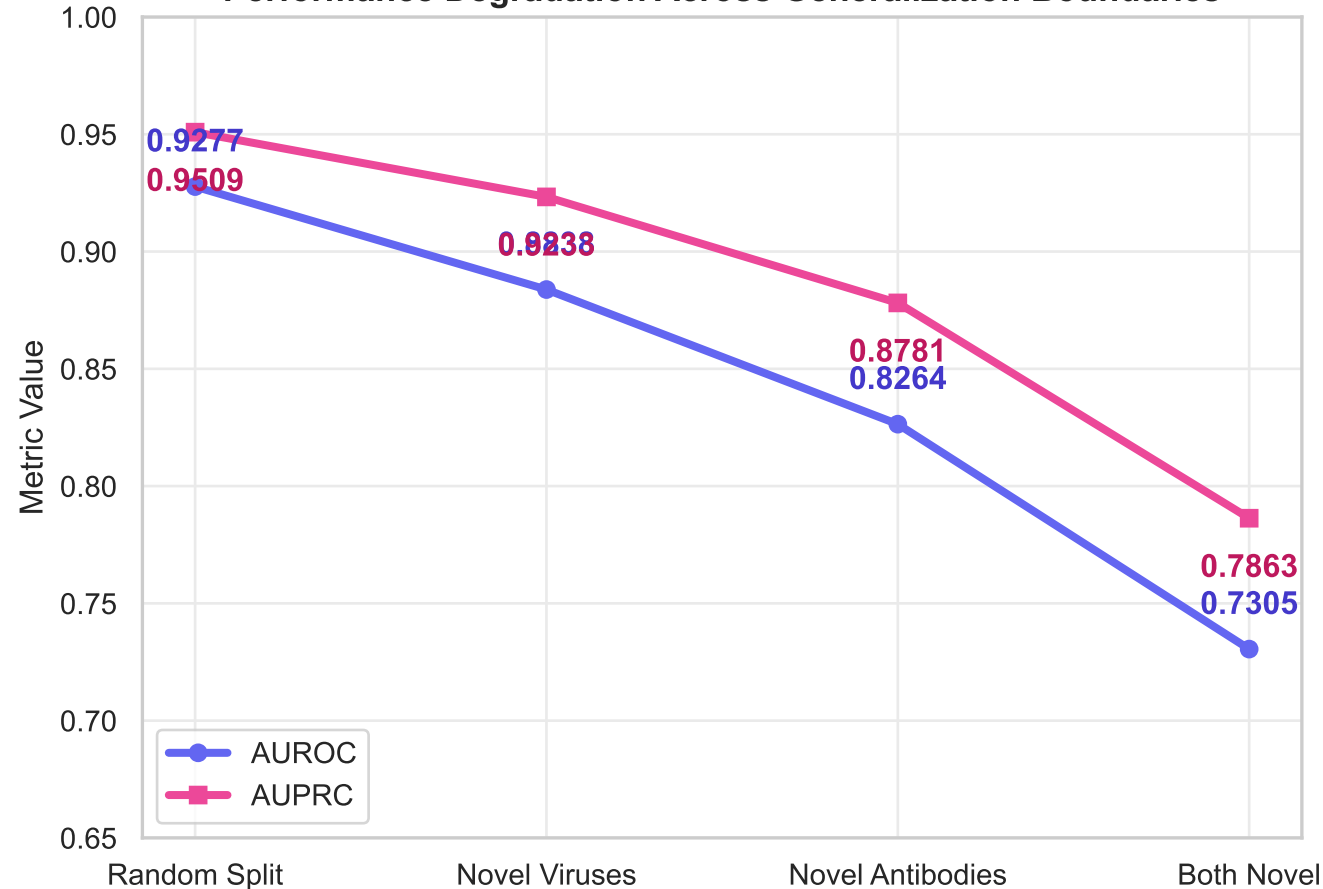
Performance Degradation Across Generalization Boundaries
