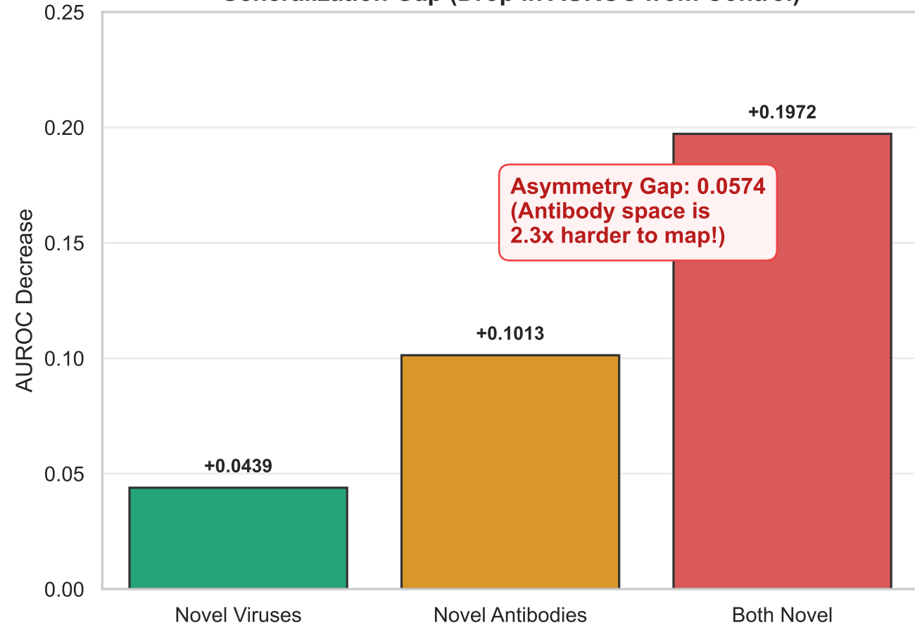
Generalization Gap (Drop in AUROC from Control)
