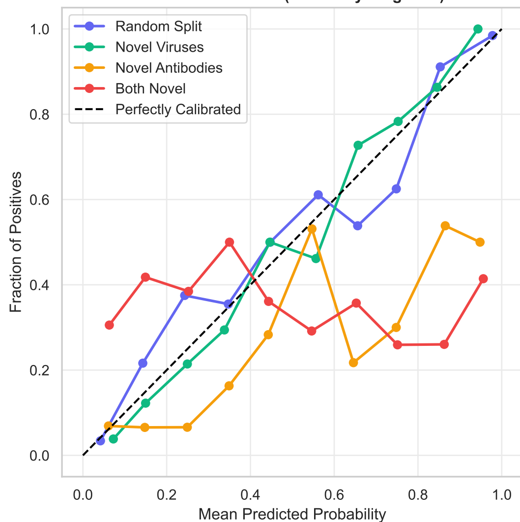
Calibration Curves (Reliability Diagrams)
