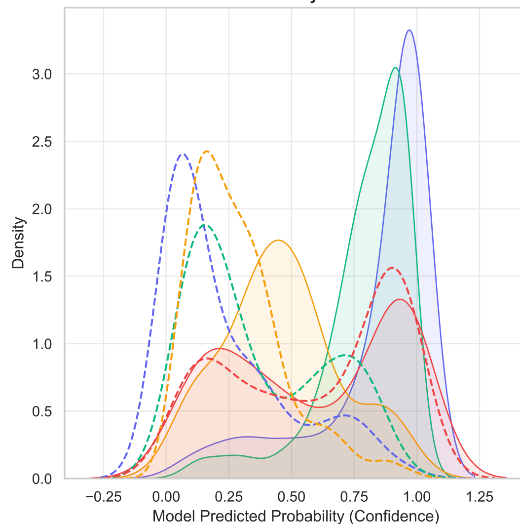
Confidence Density Distributions
