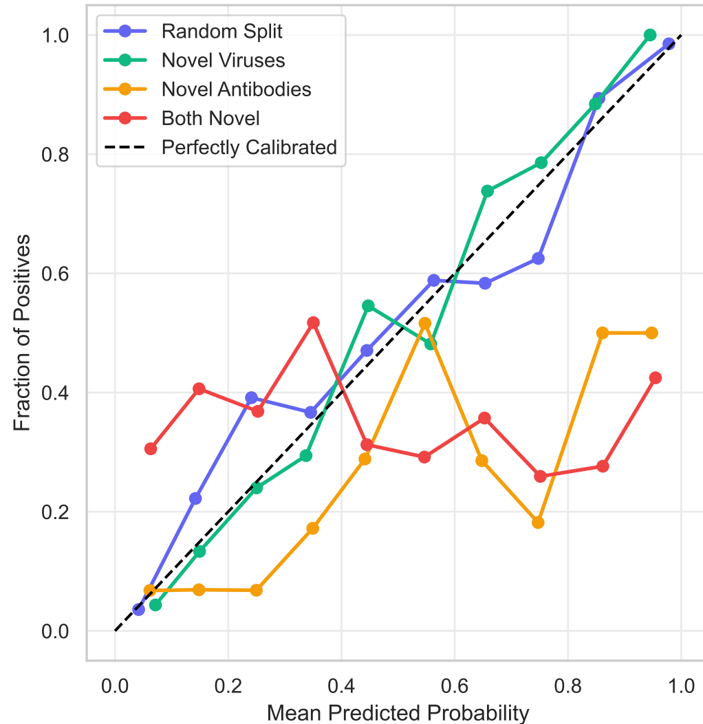
Calibration Curves (Reliability Diagrams)
