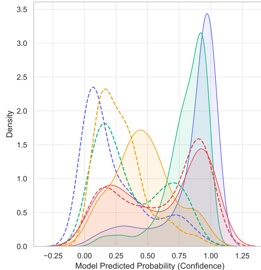
Confidence Density Distributions
