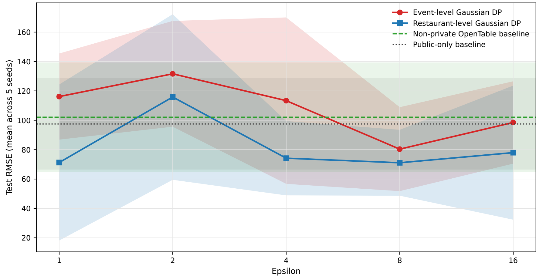
Privacy-Utility Tradeoff Across the Gaussian DP Sweep
