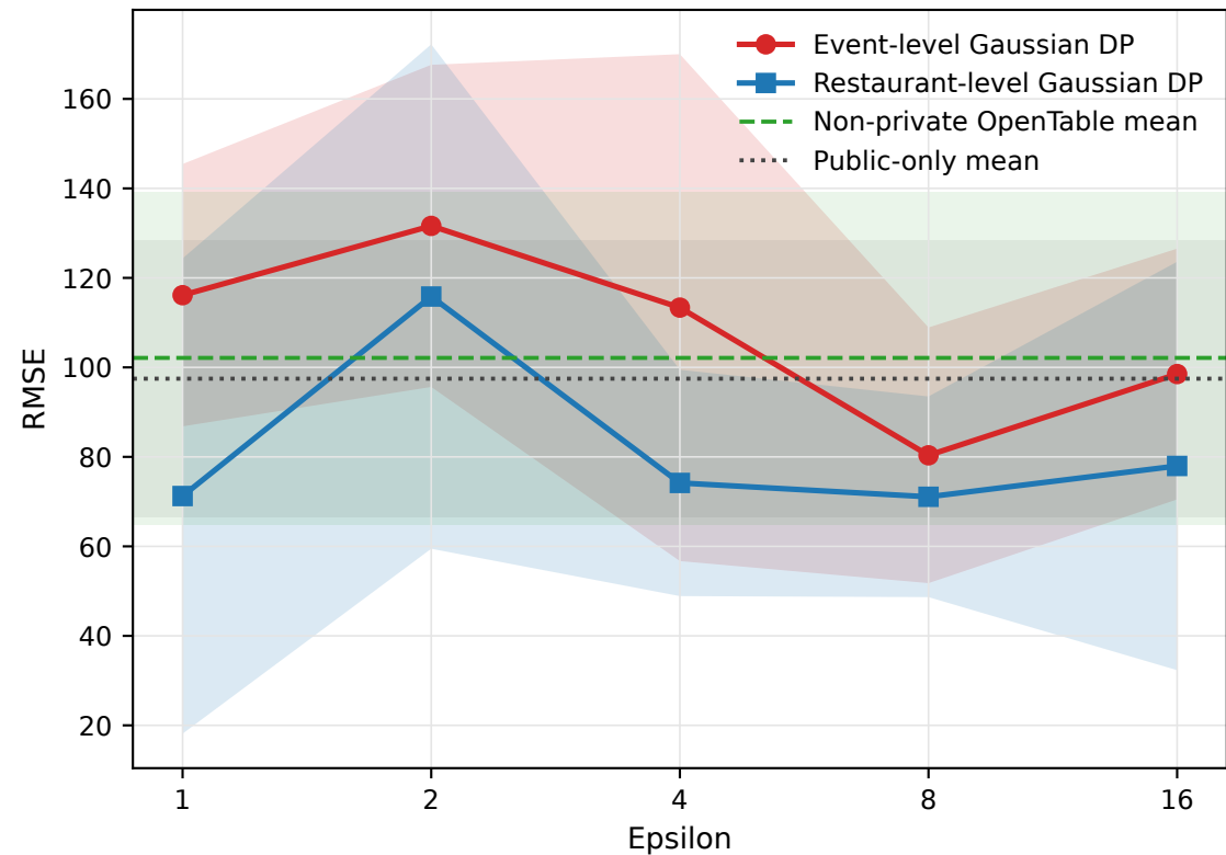
Privacy Sweep Mean RMSE Across 5 Seeds
