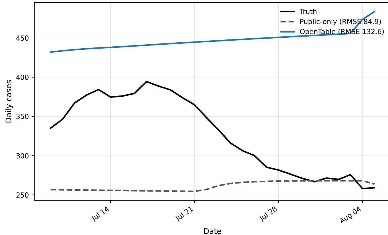
Long-Train Seed 0 Held-Out Forecast: With vs Without OpenTable
