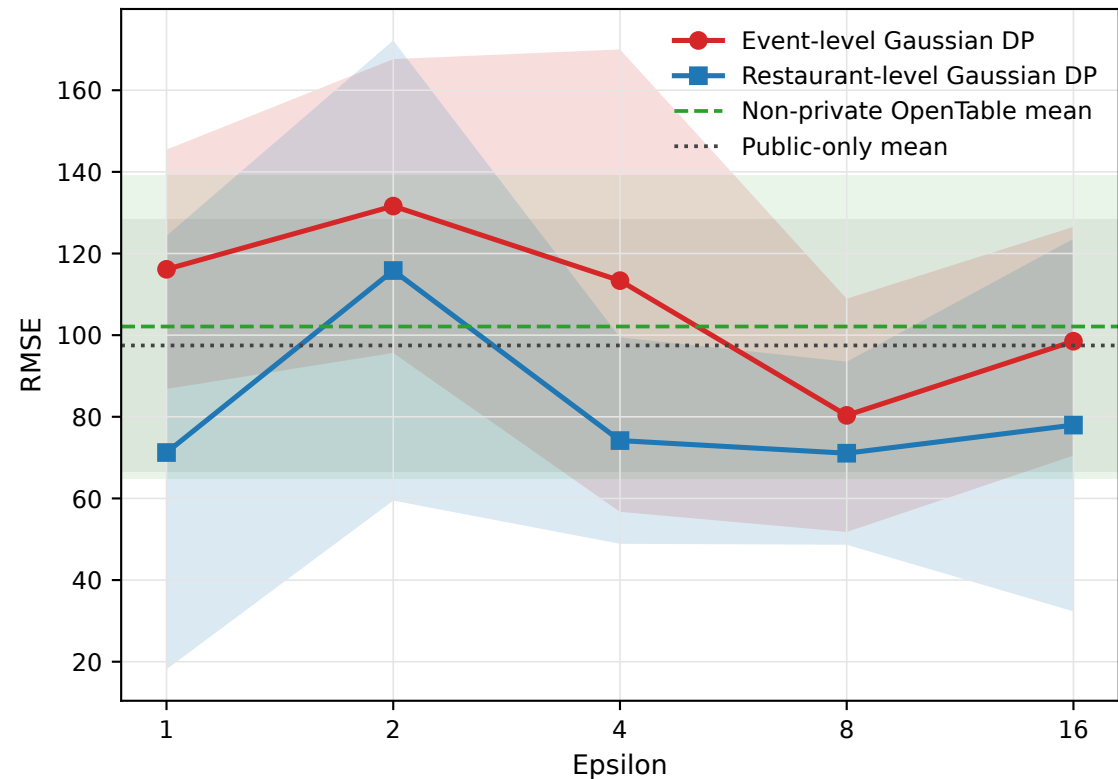
Privacy-Utility Tradeoff Across the Gaussian DP Sweep
