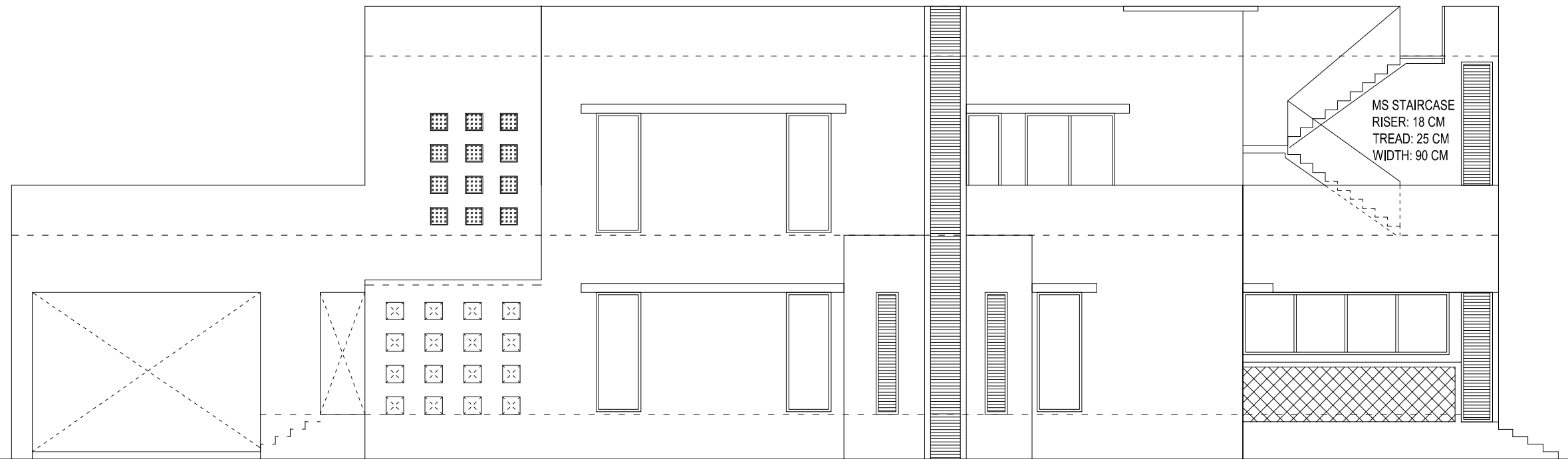
ELEVATION C
