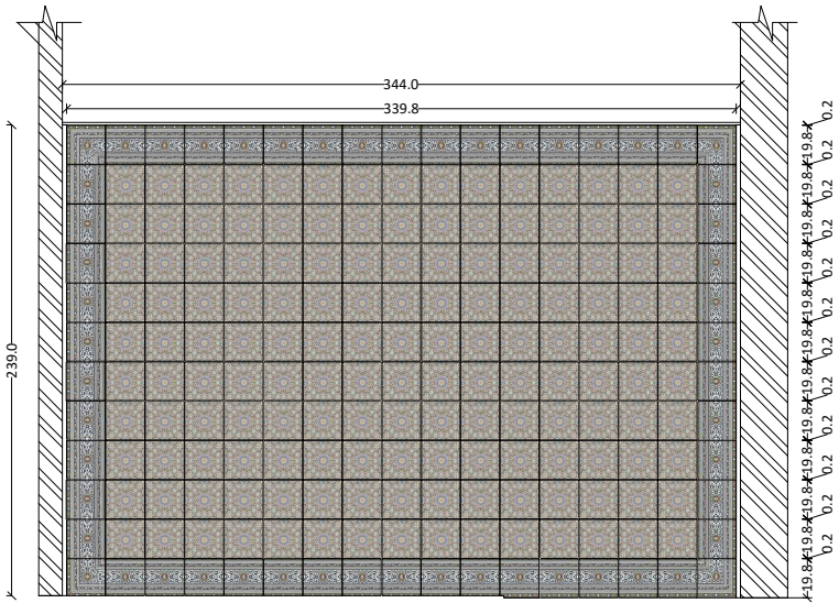
ELEVATION C
