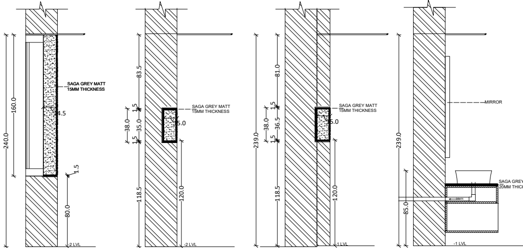
SECTION A
