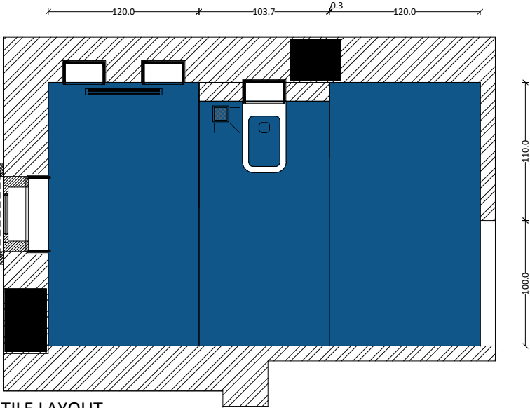
TILE LAYOUT
