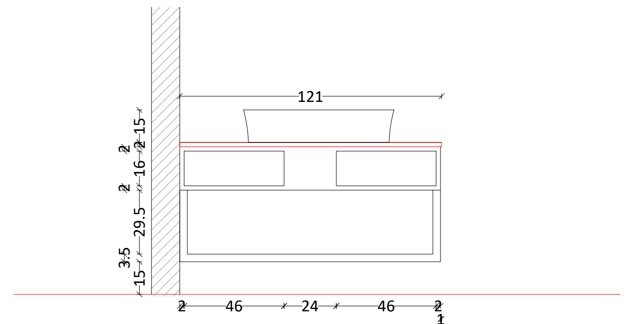
INSIDE PARTITION ELEVATION
