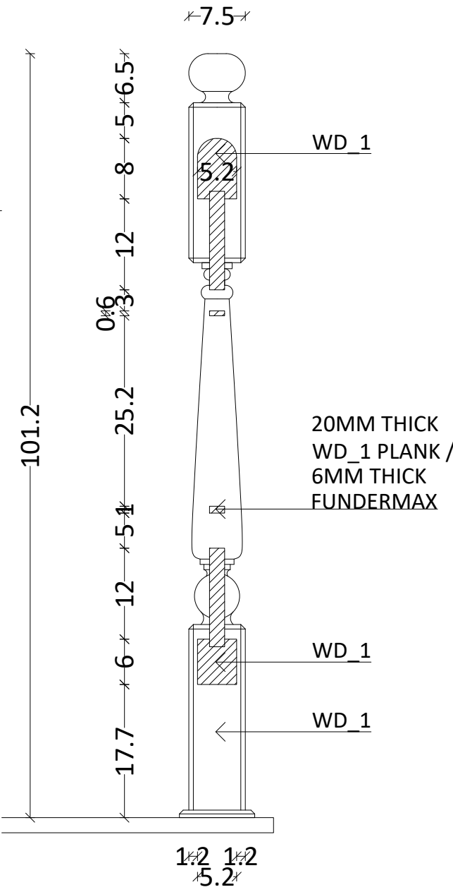
SECTION A
