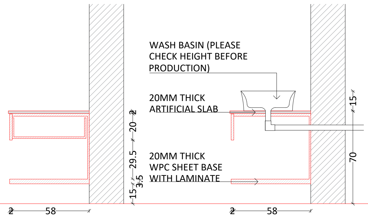
SECTION A
