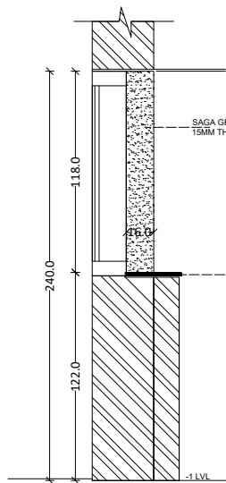
SECTION A
