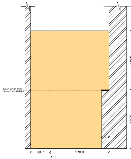
ELEVATION D
