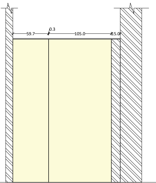
ELEVATION D
