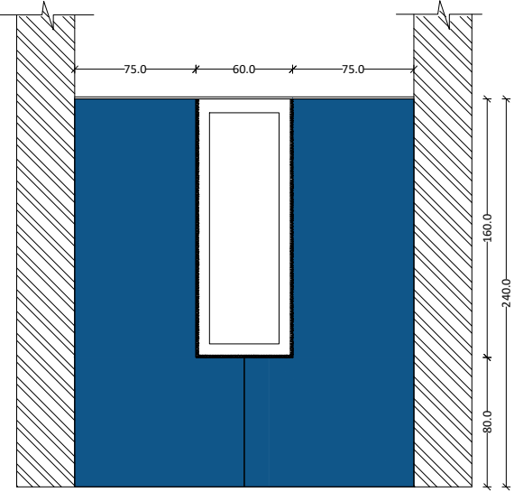
ELEVATION D
