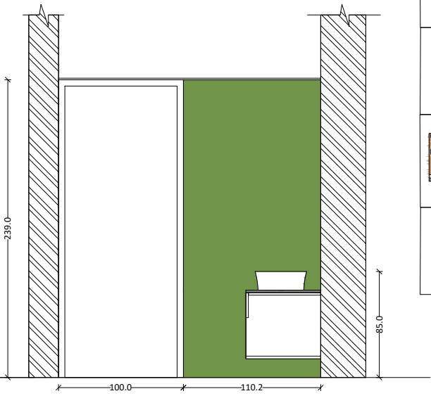
ELEVATION D
