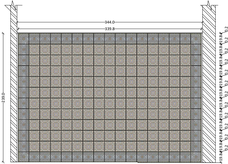
ELEVATION C
