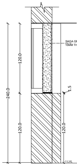
SECTION A
