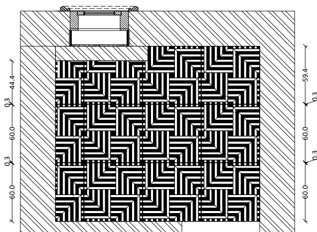
TILE LAYOUT
