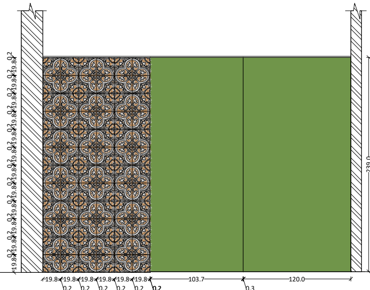
ELEVATION C
