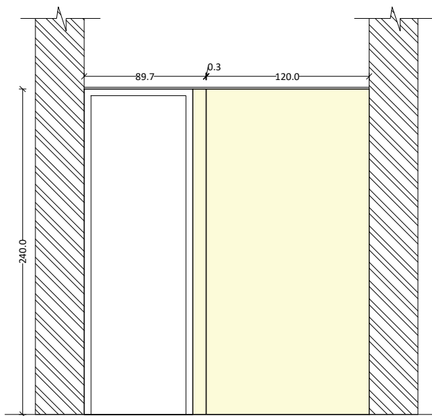
ELEVATION C
