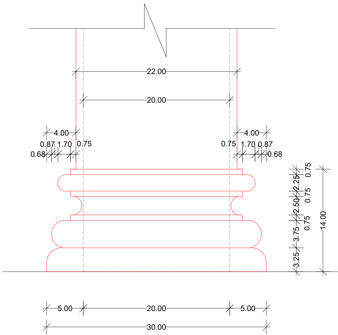
DETAIL-A
