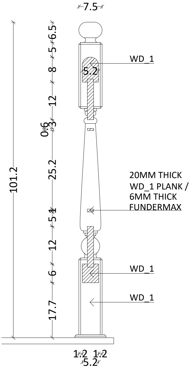
SECTION A
