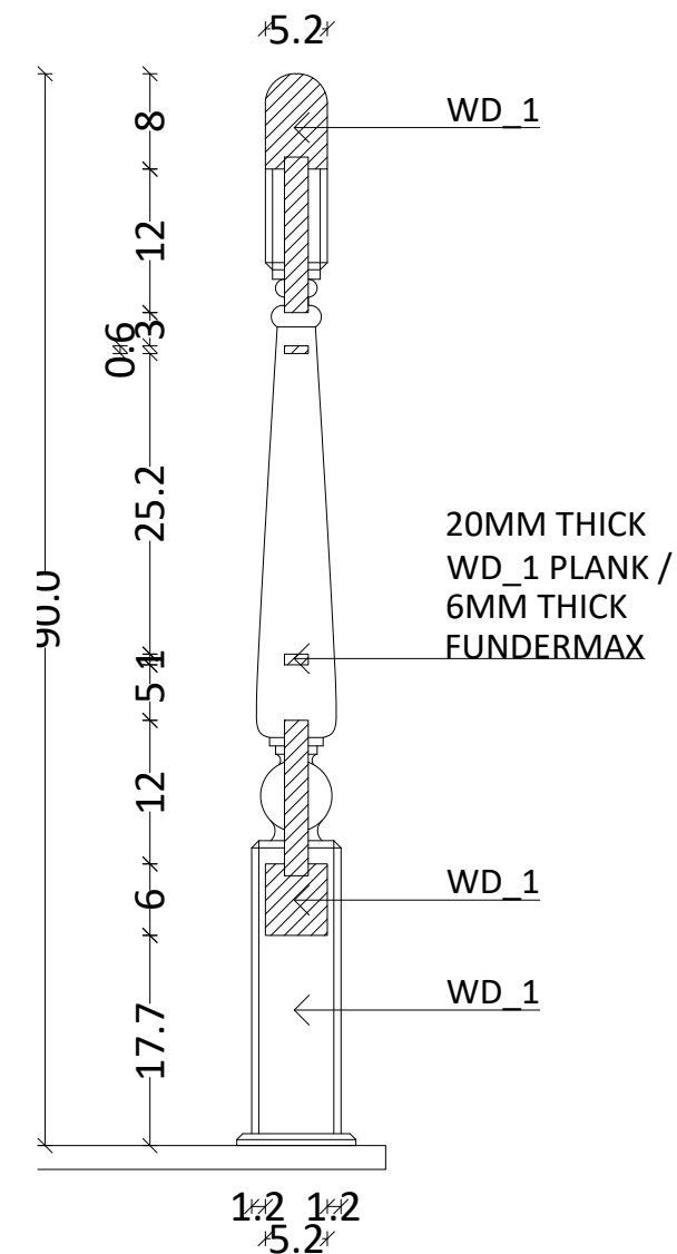
SECTION A
