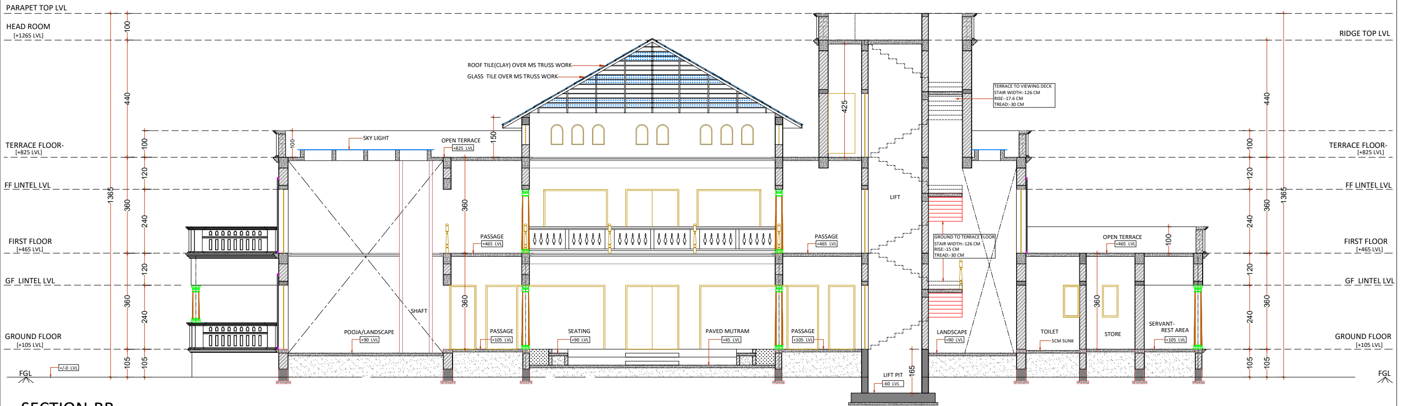
SECTION-BB
