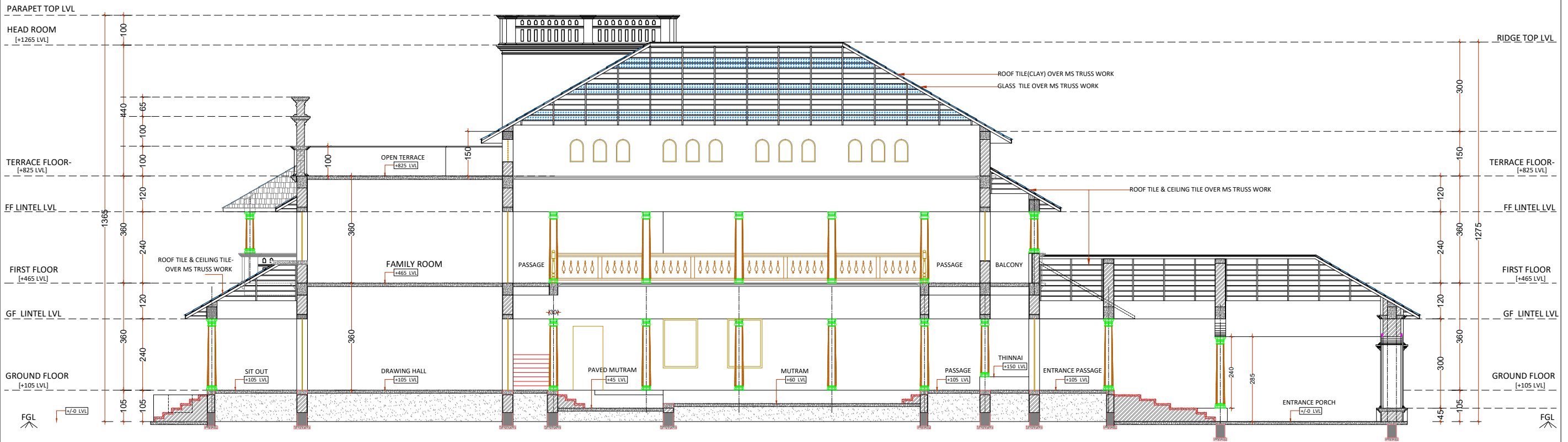
SECTION-AA
