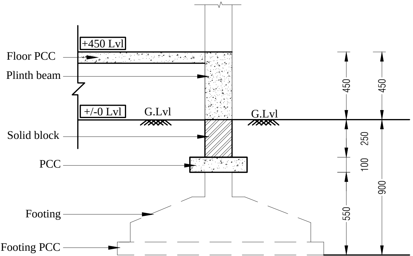
SECTION ALONG-PB(200 x 450)
