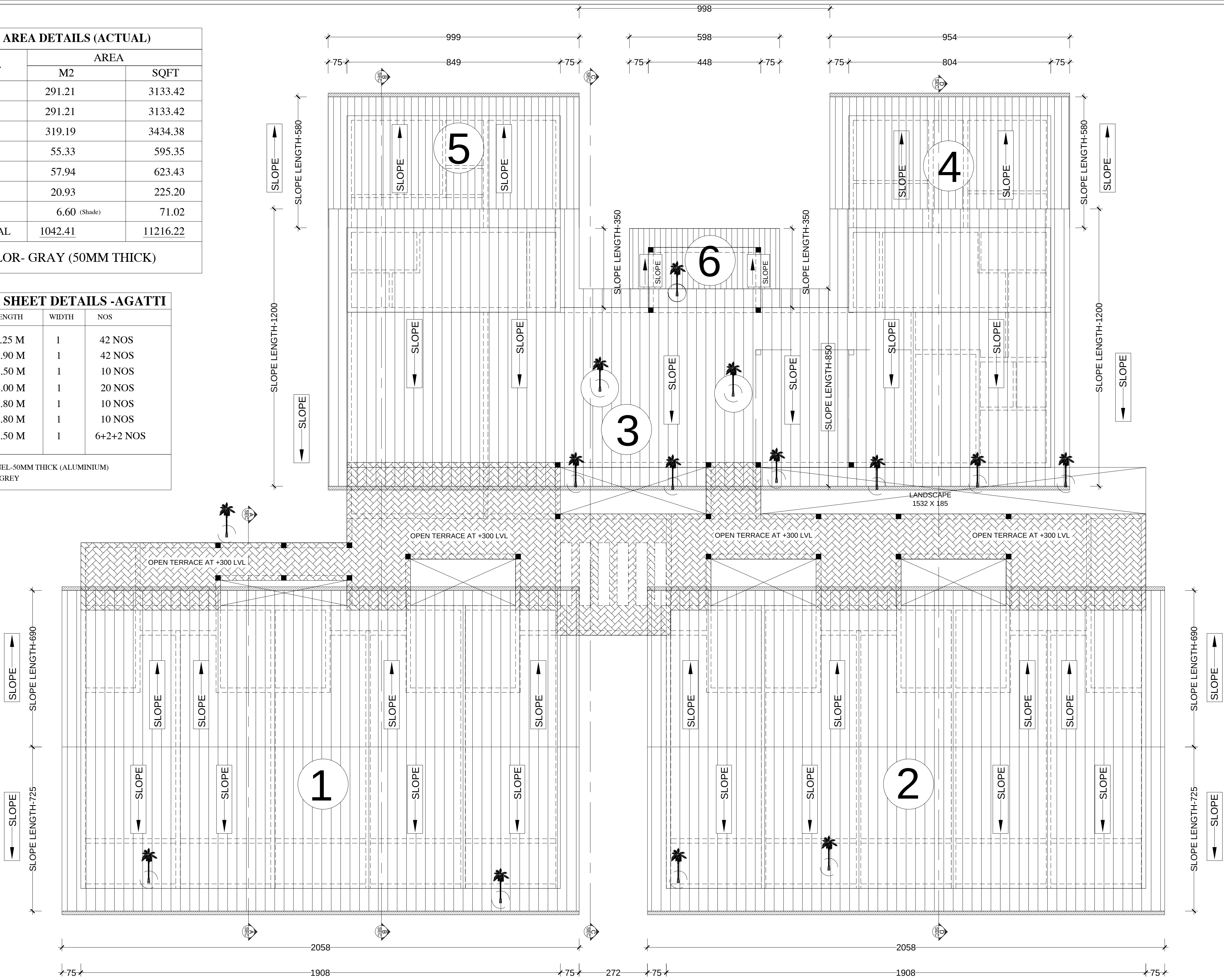
ROOF PLAN
