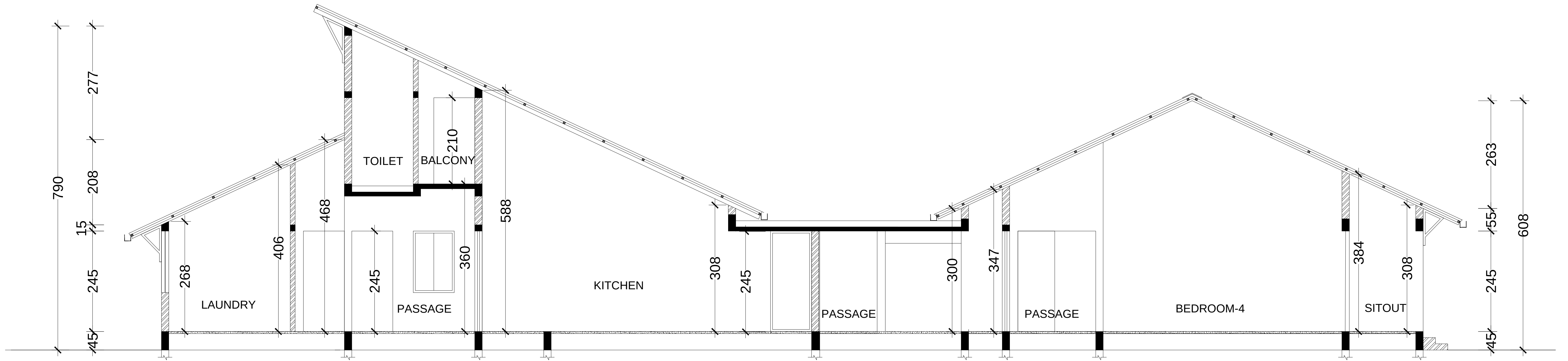
SECTION -BB
