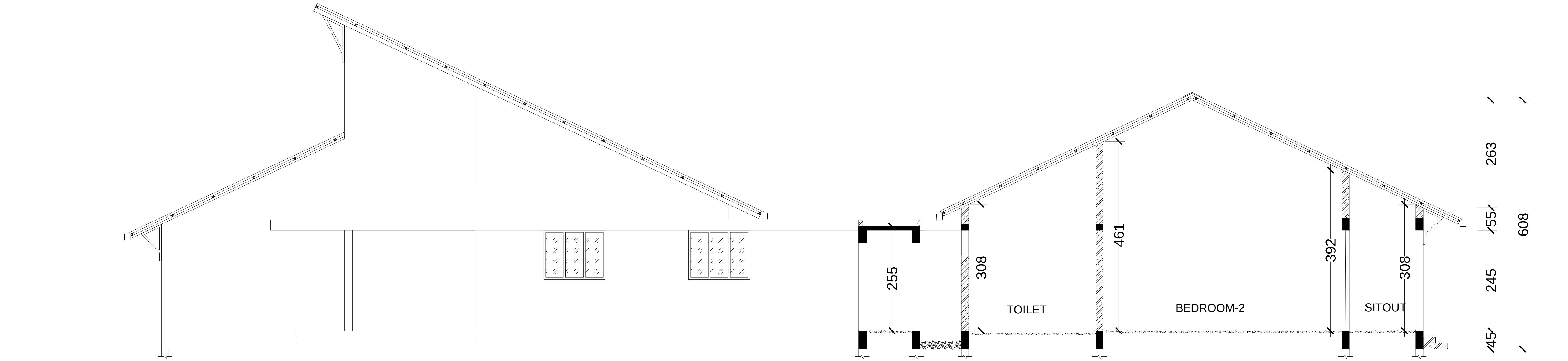
SECTION -AA
