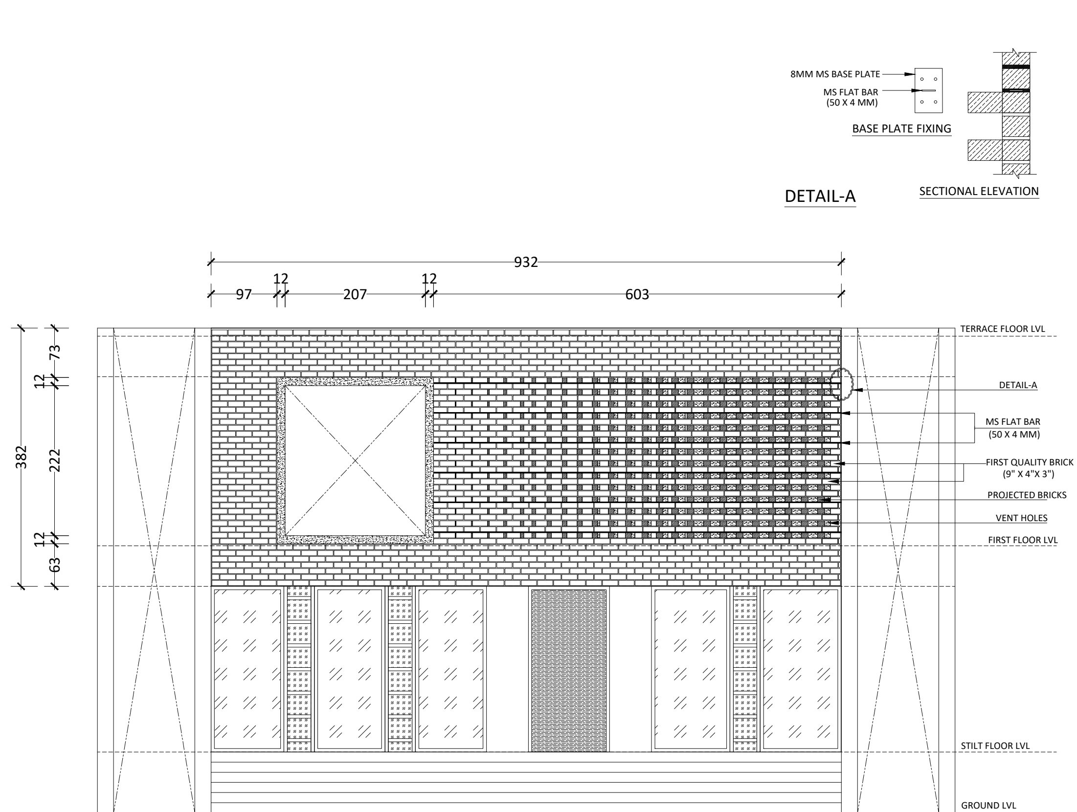
FRONT ELEVATION
