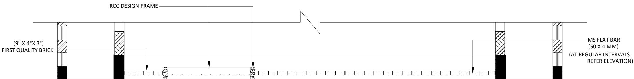
PART PLAN
