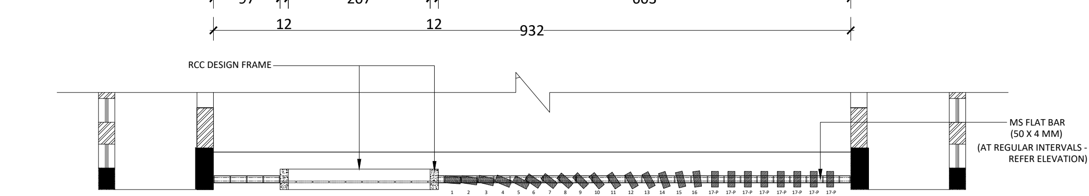
PART PLAN(Projected brick laying)
