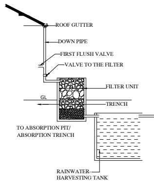
SCHEMATIC SECTION
