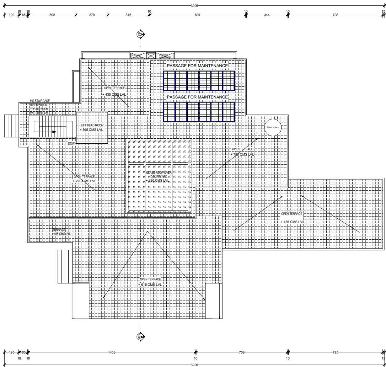
TERRACE FLOOR SCALE 1:100
