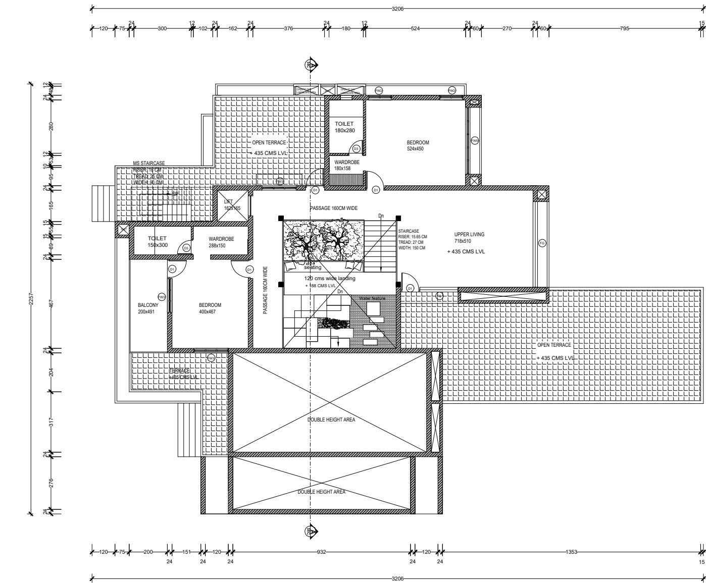
FIRST FLOOR SCALE 1:100
