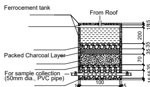
CROSS SECTION ON BB
