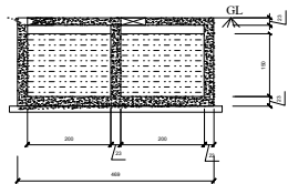
SECTION PP
