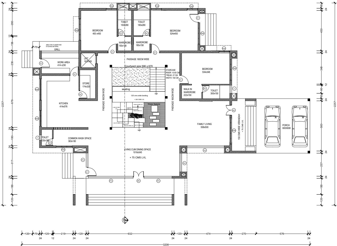
GROUND FLOOR
