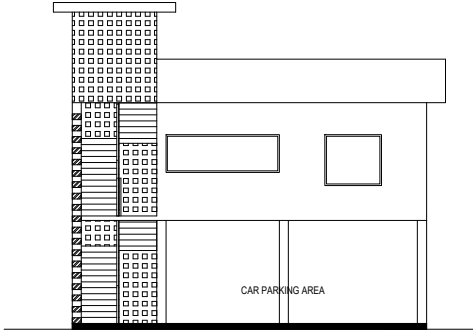
OUTHOUSE ELEVATION
