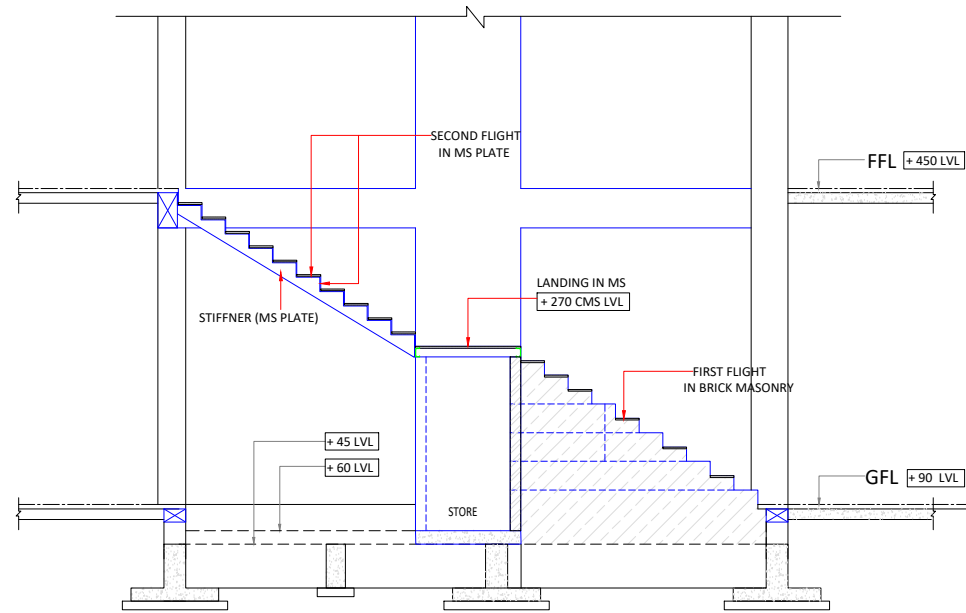
PART SECTION-XX
