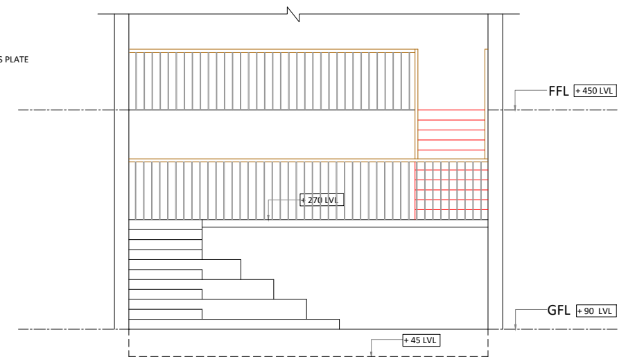
PART ELEVATION
