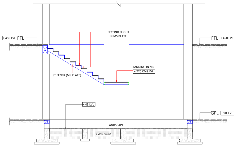
PART SECTION-YY
