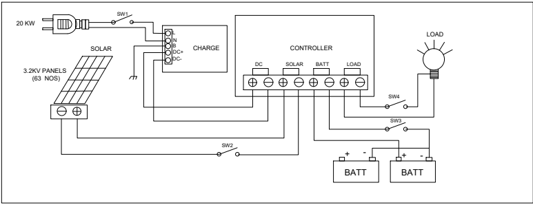
SOLAR ELECTIC POWER GENERATING SYSTEM NTS
