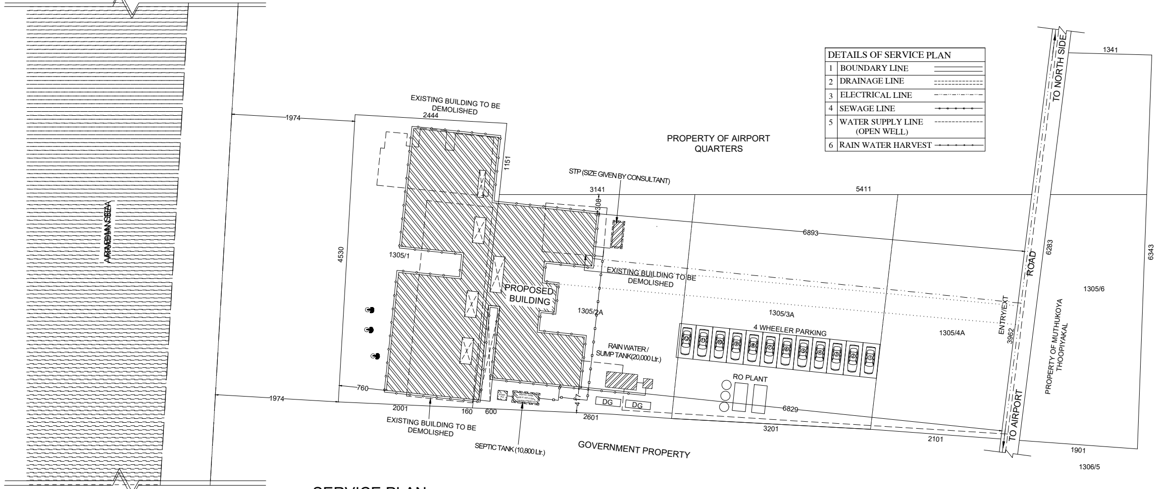
SERVICE PLAN SCALE 1:1300
