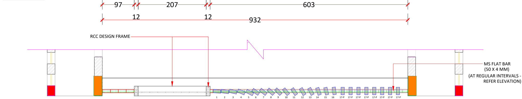
PART PLAN(Projected brick laying)
