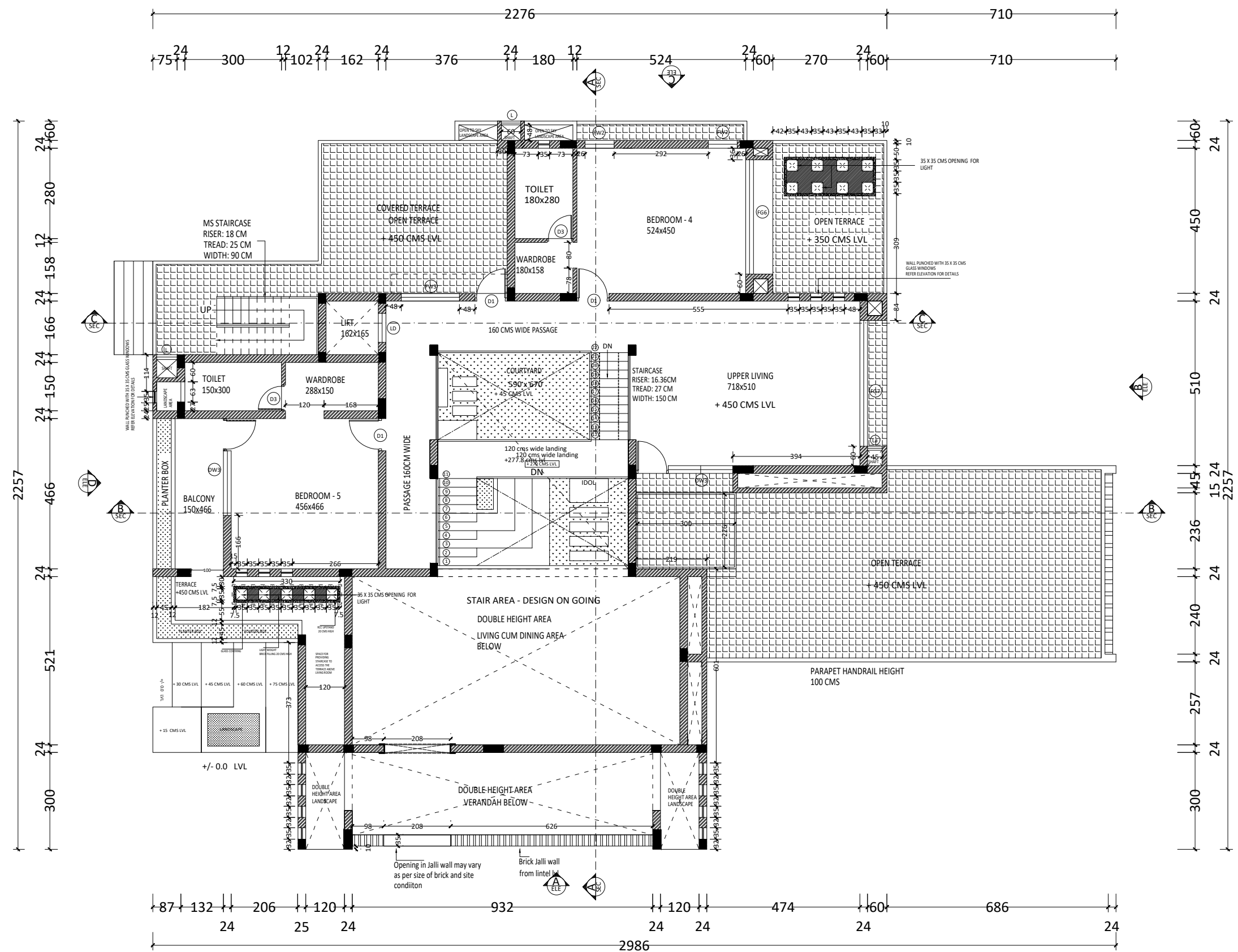
FIRST FLOOR
