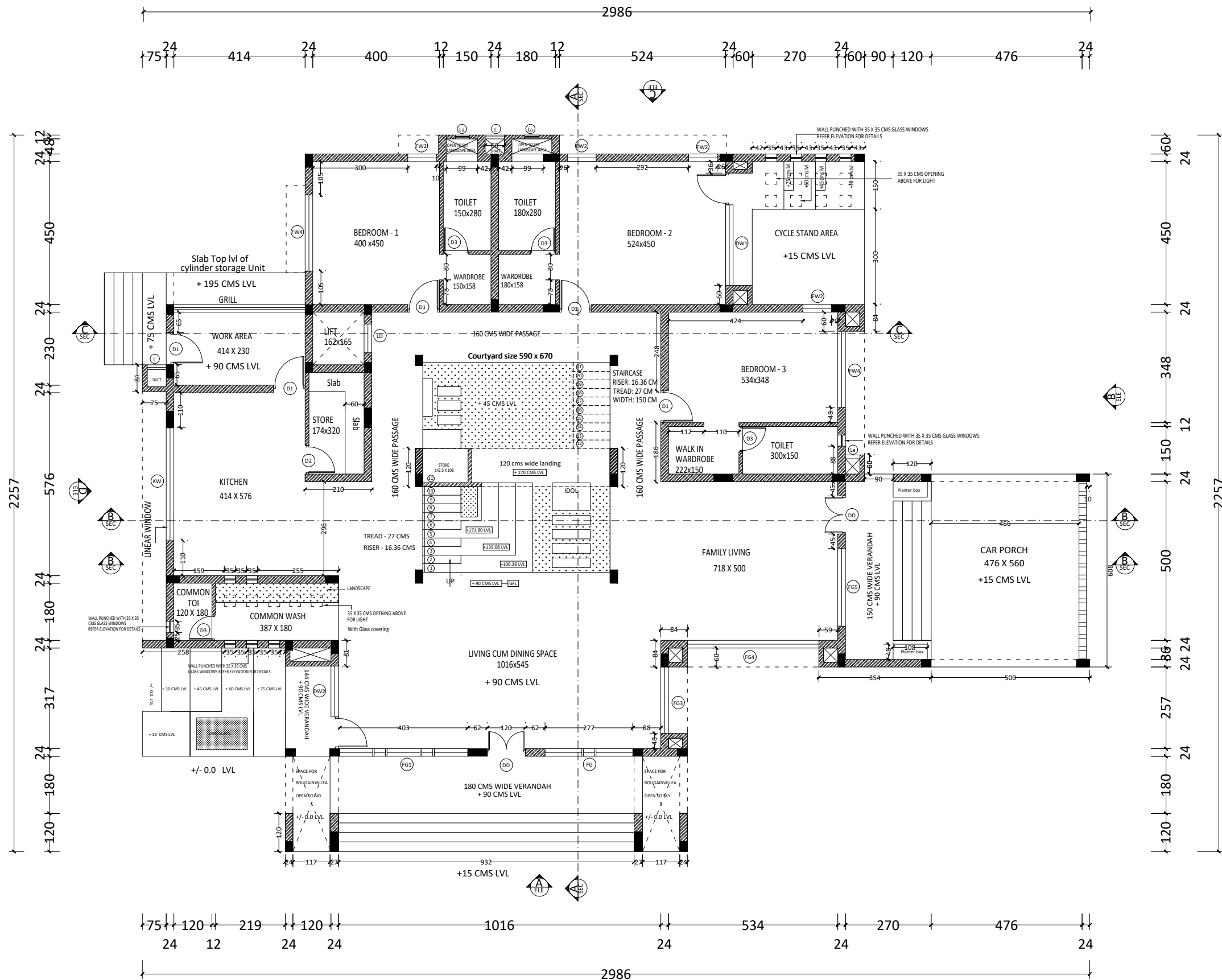
GROUND FLOOR
