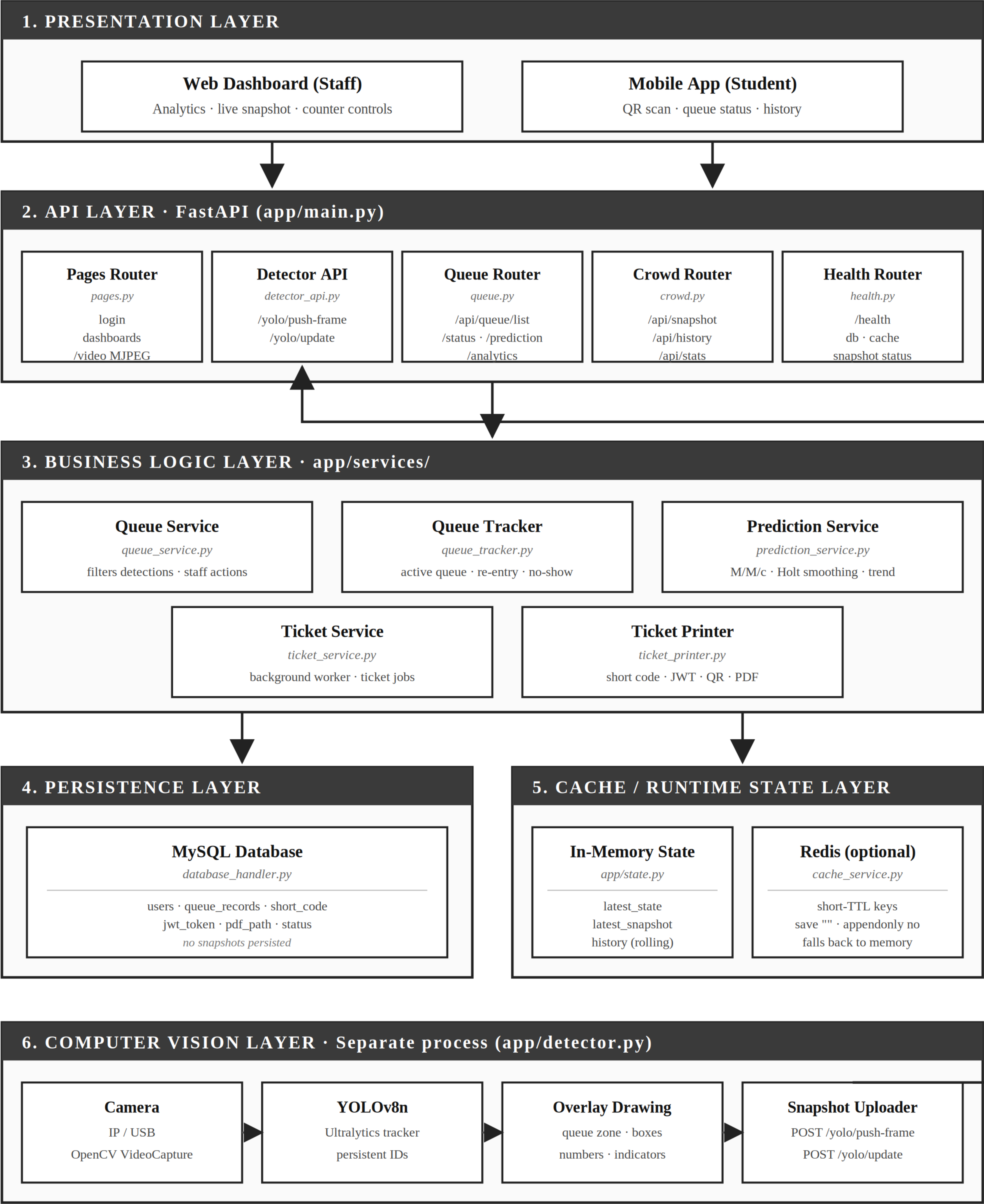
Figure 2.1. QueueFlow six-layer system architecture.
