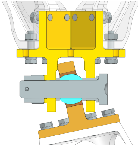
Figure 6: GMA - yaw=12°, pitch=0°
