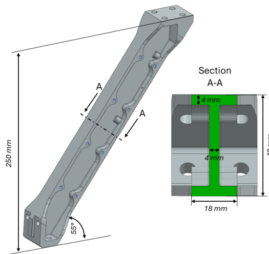
Figure 7: Thrust Frame Beam dimensions
