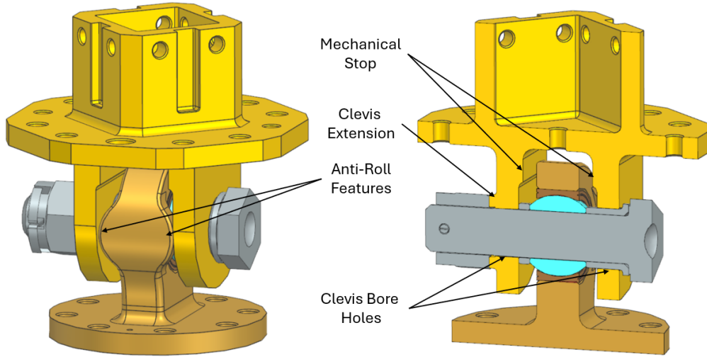
Figure 5: Chosen features of GMA parts
