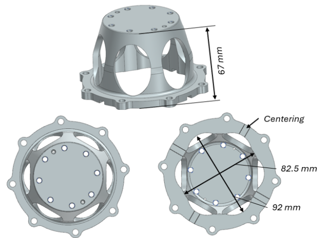
Figure 8: Thrust Dome design
