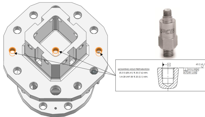
Figure 7: Shock-accelerometer mounting interface
