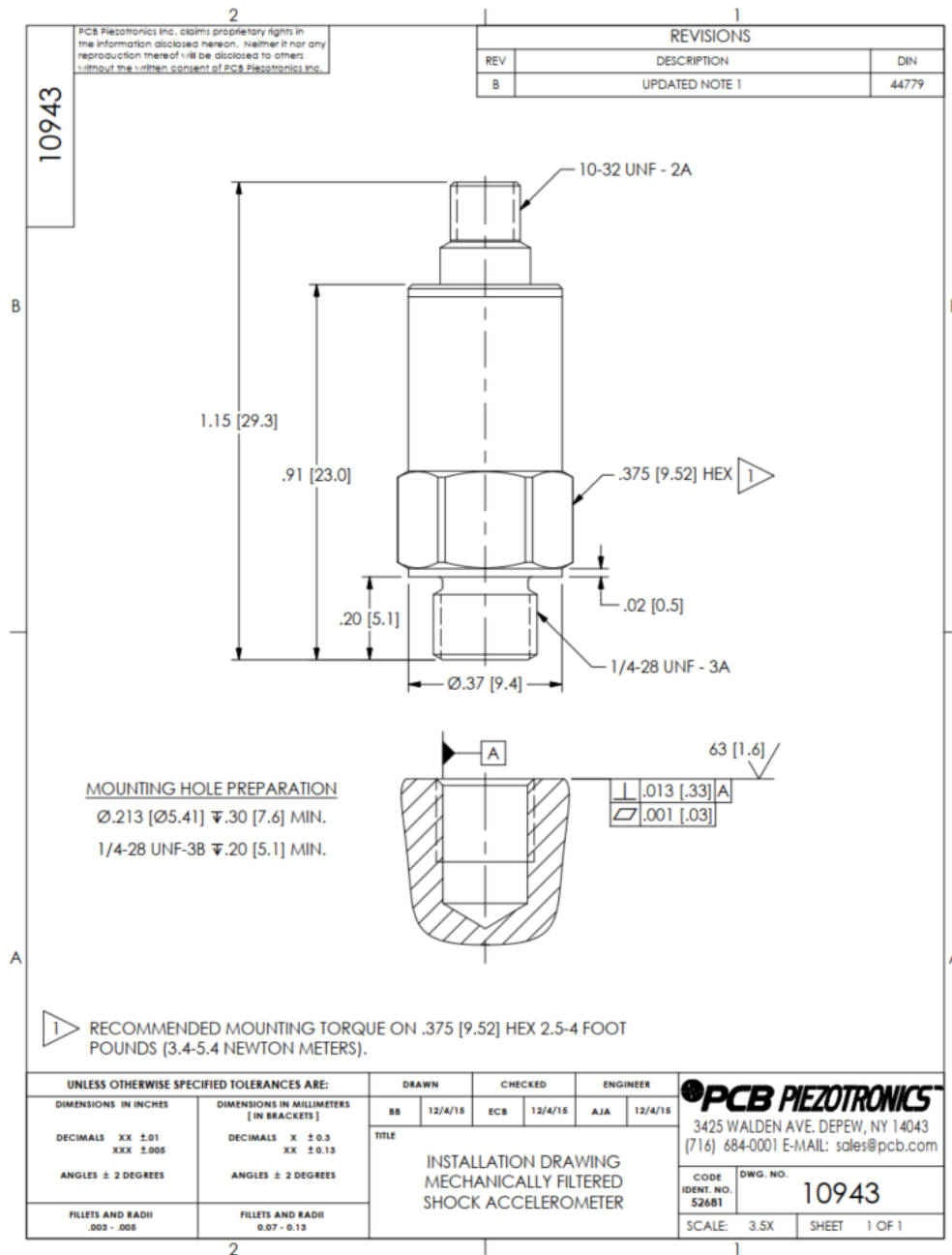
Figure 10: Installation drawing of shock accelerometer [RD3]
