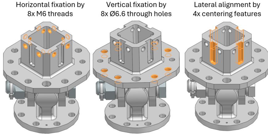
Figure 4: Interfaces between GMA and Thrust Frame Beams
