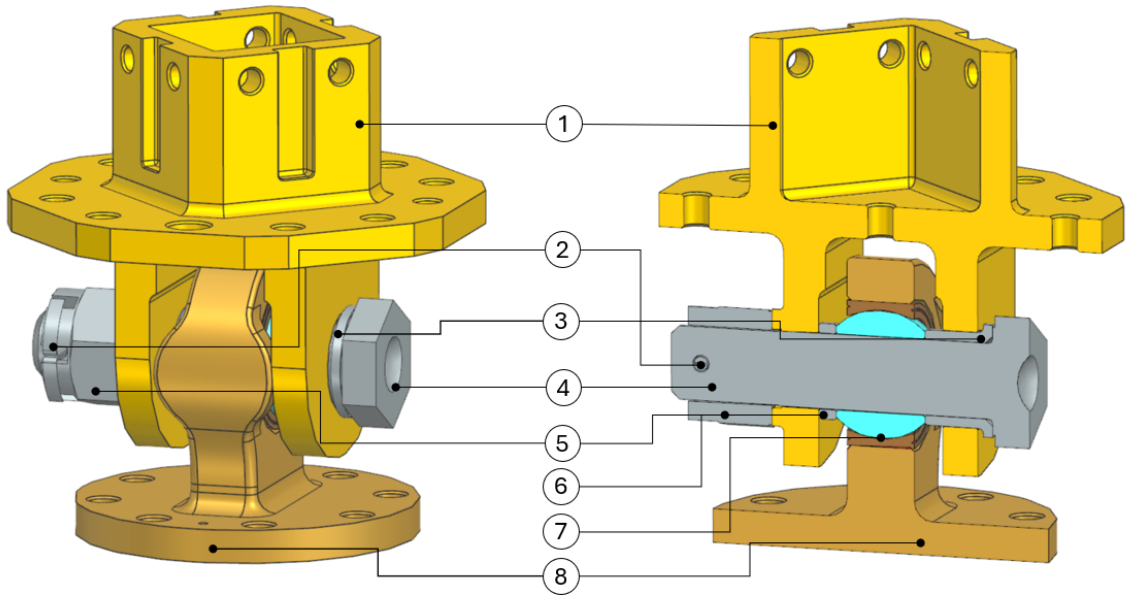
Figure 4: GMA isometric view and cross section
