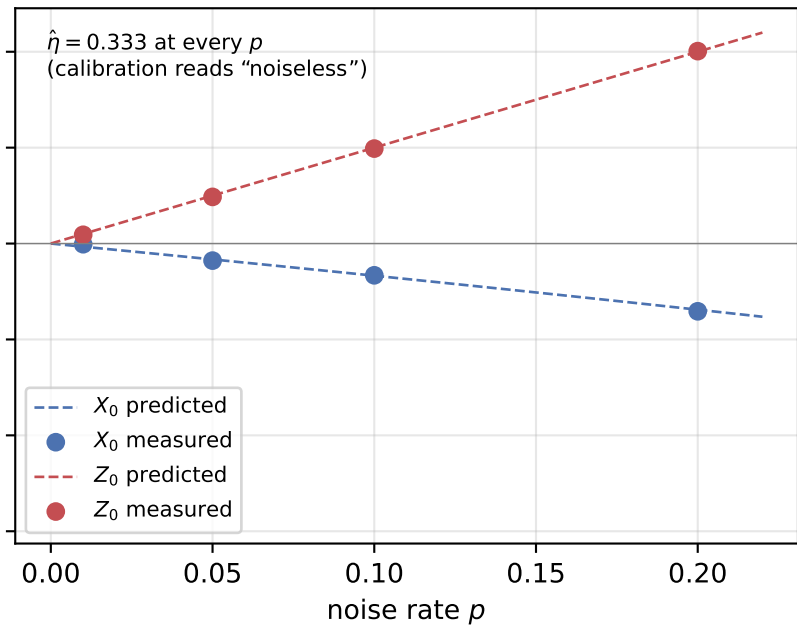
(b) amplitude damping
