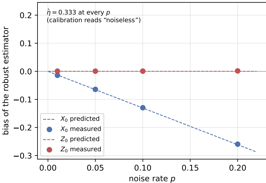
(a) dephasing
