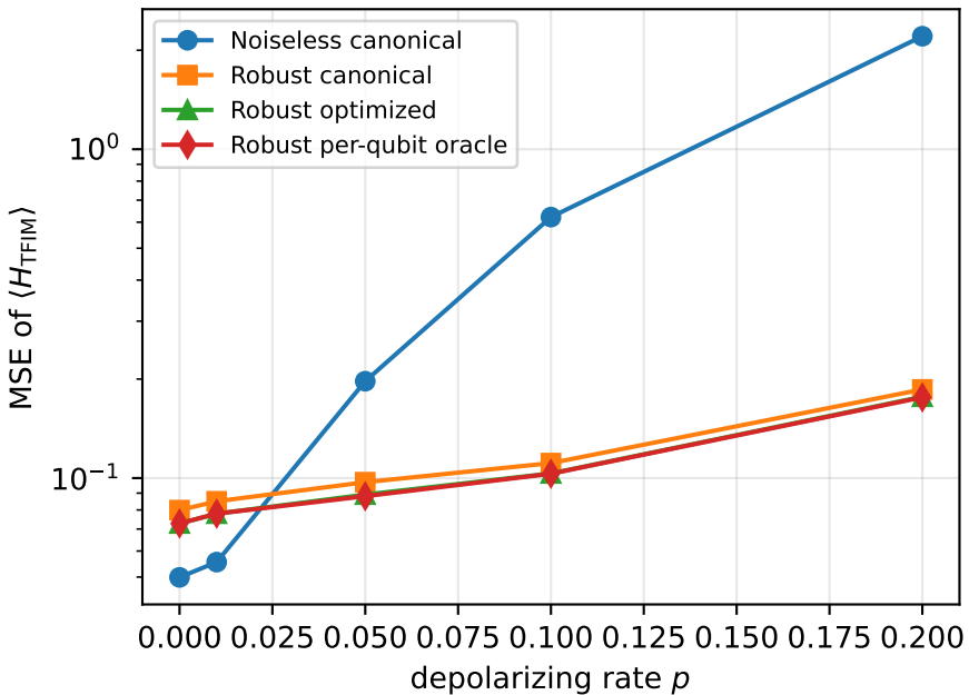
(a) estimator hierarchy under noise
