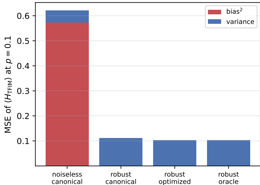
(b) bias converted to variance
