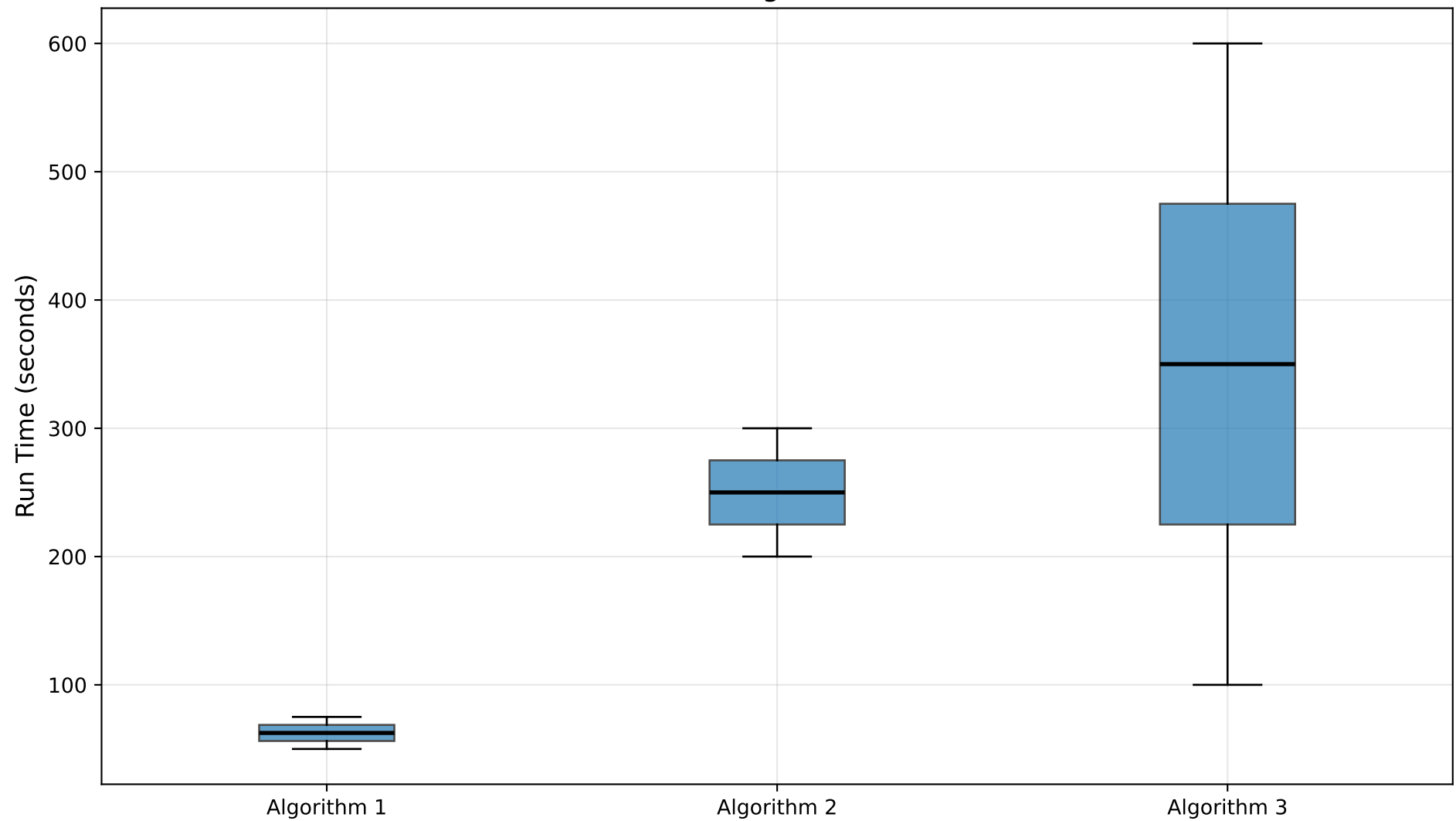
Distribution of Algorithm Run Times
