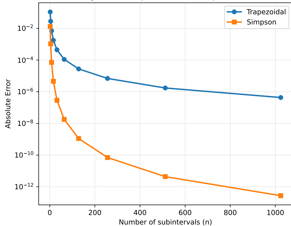
Convergence of Trapezoidal and Simpson Methods
