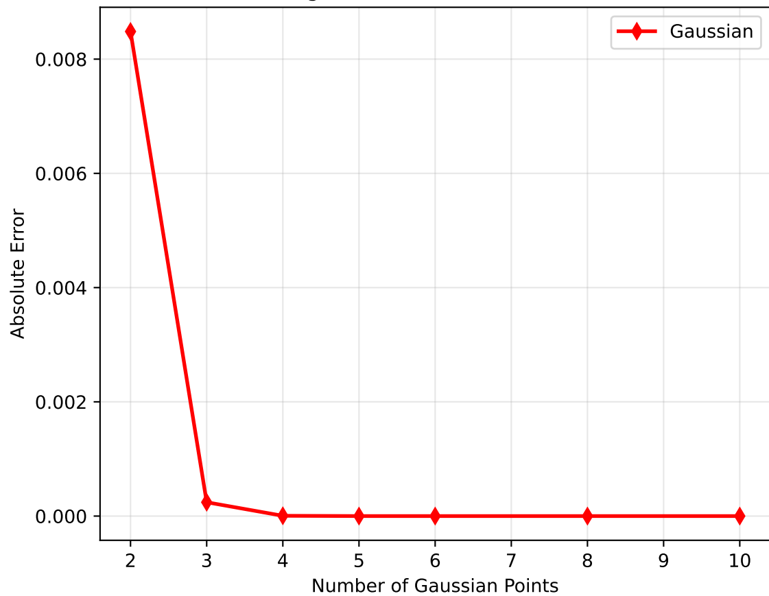
Convergence of Gaussian Quadrature
