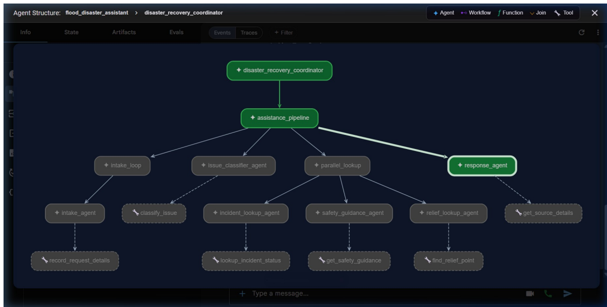
Figure F1. ADK Web Agent Structure: LLM, Sequential, Parallel and Loop agents with the registered Function tools
