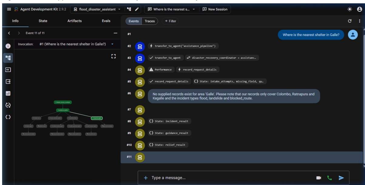
Figure F5b. Not-found result for Galle; later stages skipped
