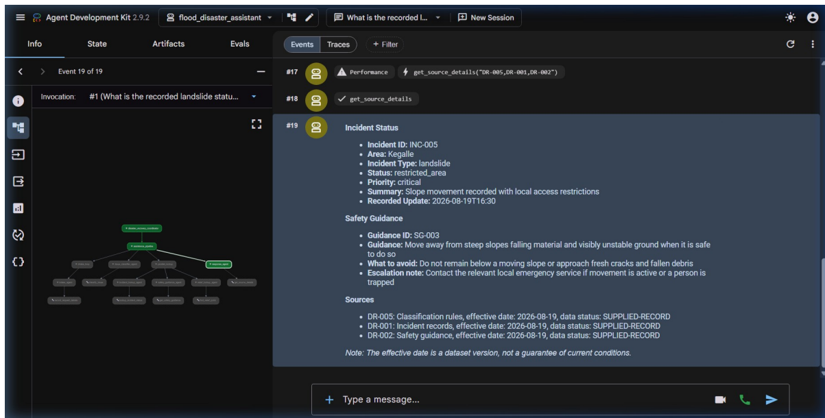
Figure F2. Events trace (final events #17 to #19) and workflow graph for the Kegalle landslide request
