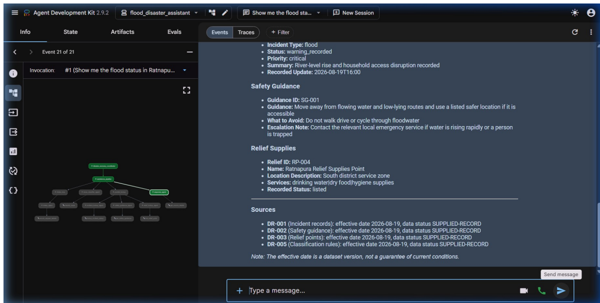
Figure F3. Combined answer with incident, safety guidance and relief branch results
