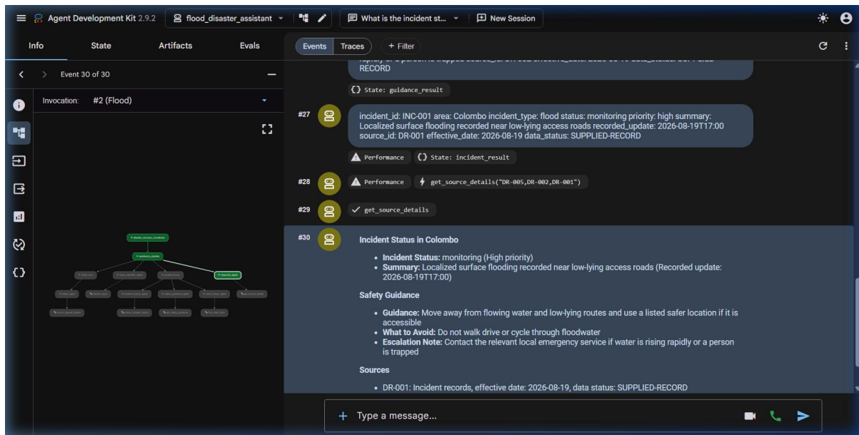
Figure F4. Invocation #2 ("Flood"): the workflow continued after the missing value was supplied
