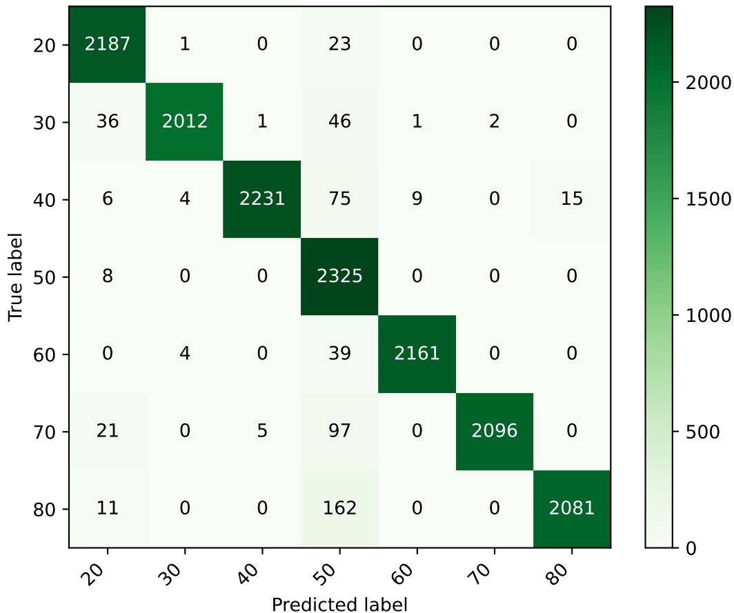
Confusion Matrix - RF(Validation)
