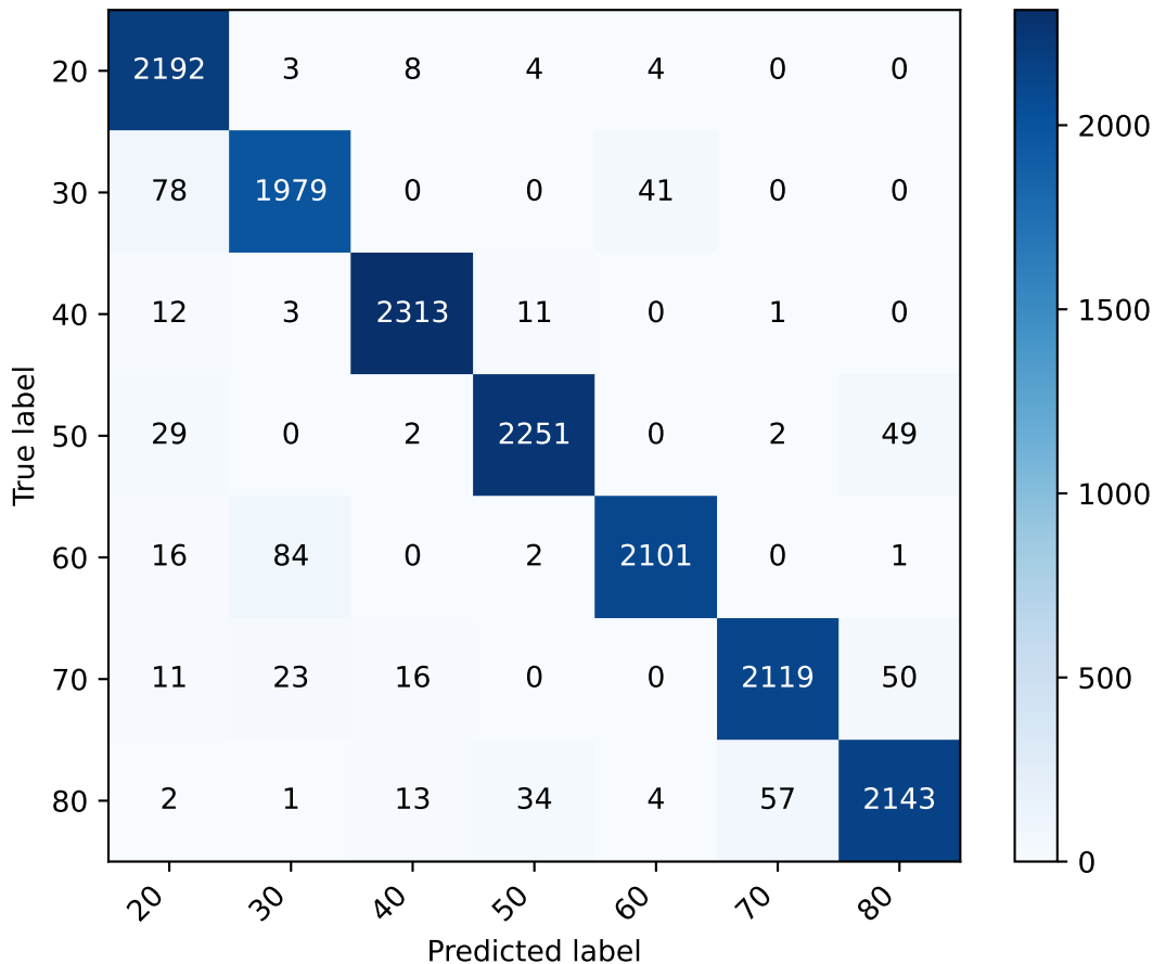
Confusion Matrix - SVM(Validation)
