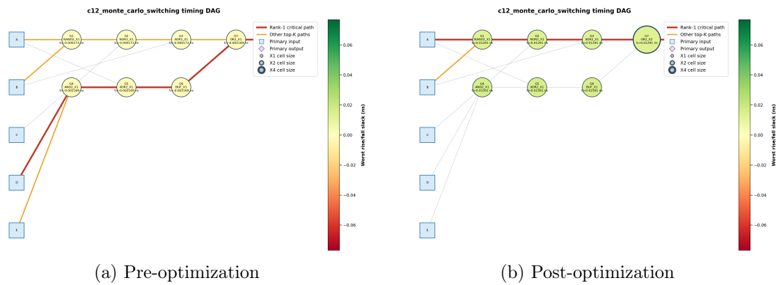
Figure B.34: c12_monte_carlo_switching: circuit diagrams, nodes colored by slack, critical path highlighted.
