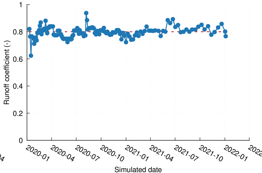
(b) Runoff coefficient: held at stationary truth
