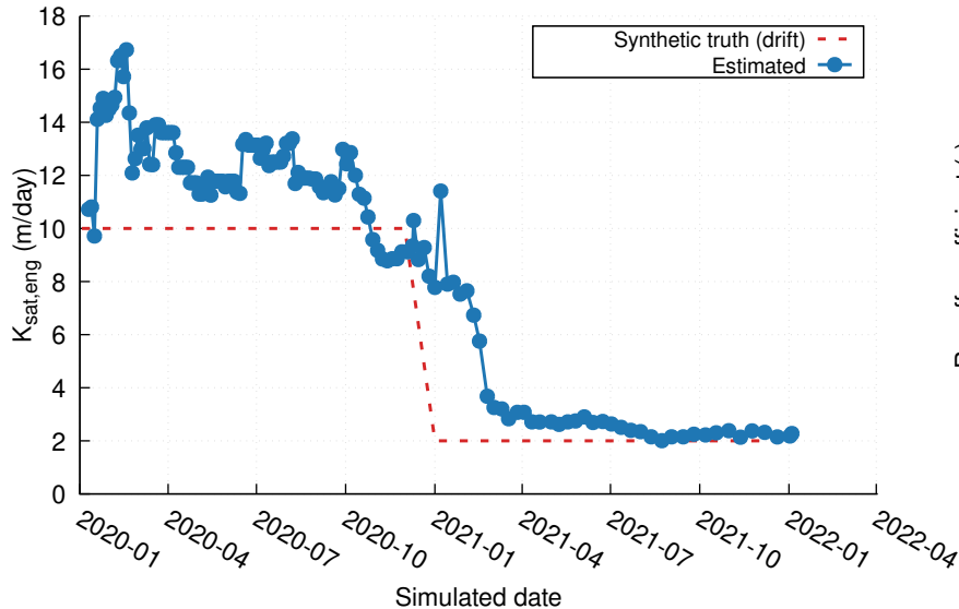
(a) Engineered-soil conductivity: tracks imposed drift
