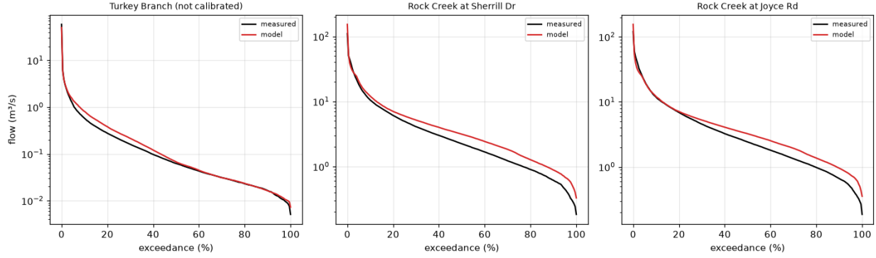
Figure 23: Flow-duration curves, WY2020–2025.
