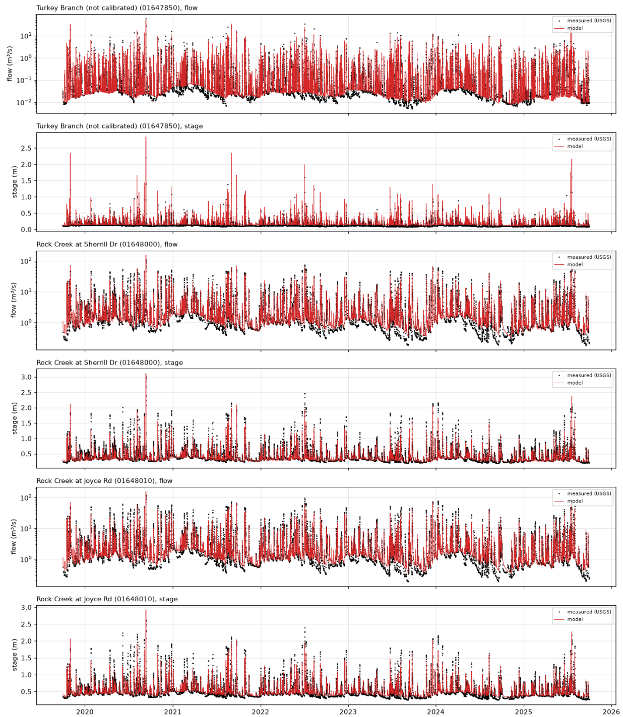
Figure 22: Validation, WY2020–2025: measured (USGS, black) and modelled (red) flow (log scale) and stage.
