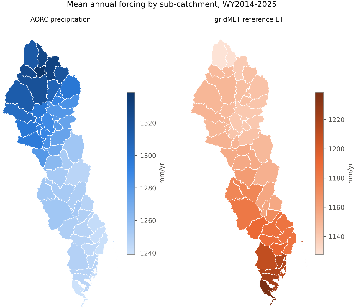
Figure 21: Mean annual AORC precipitation and gridMET reference ET by sub-catchment, WY2014–2025.
