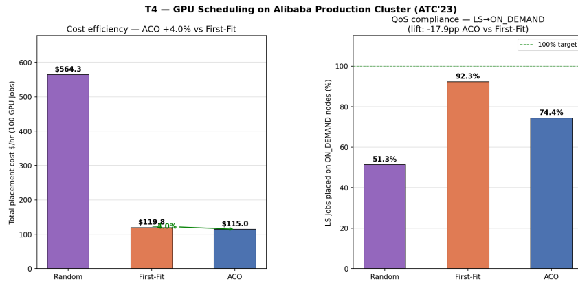
Fig. 5. T4.1 — GPU scheduling on the Alibaba production cluster (ATC’23). Left: total placement cost (100 GPU jobs). Right: LS job placement on ON_DEMAND nodes (%).
