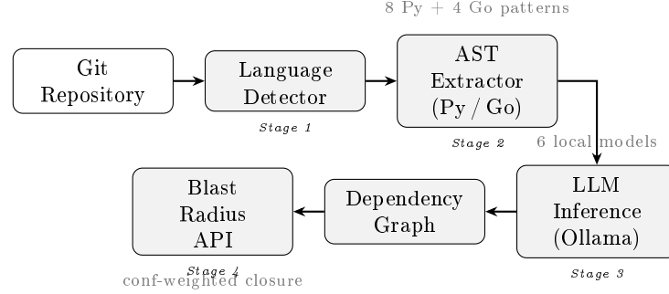
Fig. 1. The SERVICESCOPE four-stage pipeline. A cloned repository passes through language detection, AST extraction, local LLM inference, and graph-based blast radius computation.
