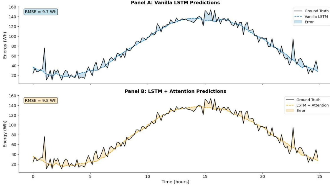
Figure 3: Model predictions vs ground truth.
