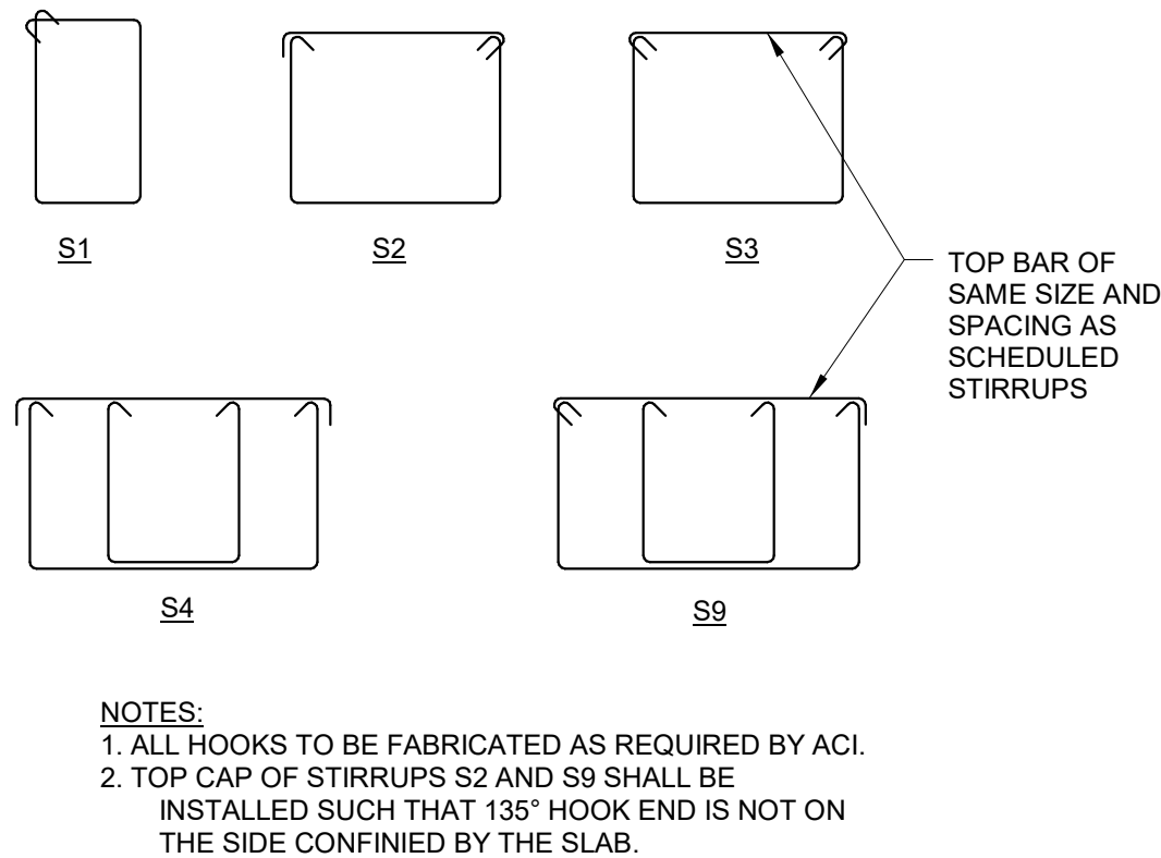
5 TYPICAL STIRRUP TYPES 3/4" = 1'-0"
