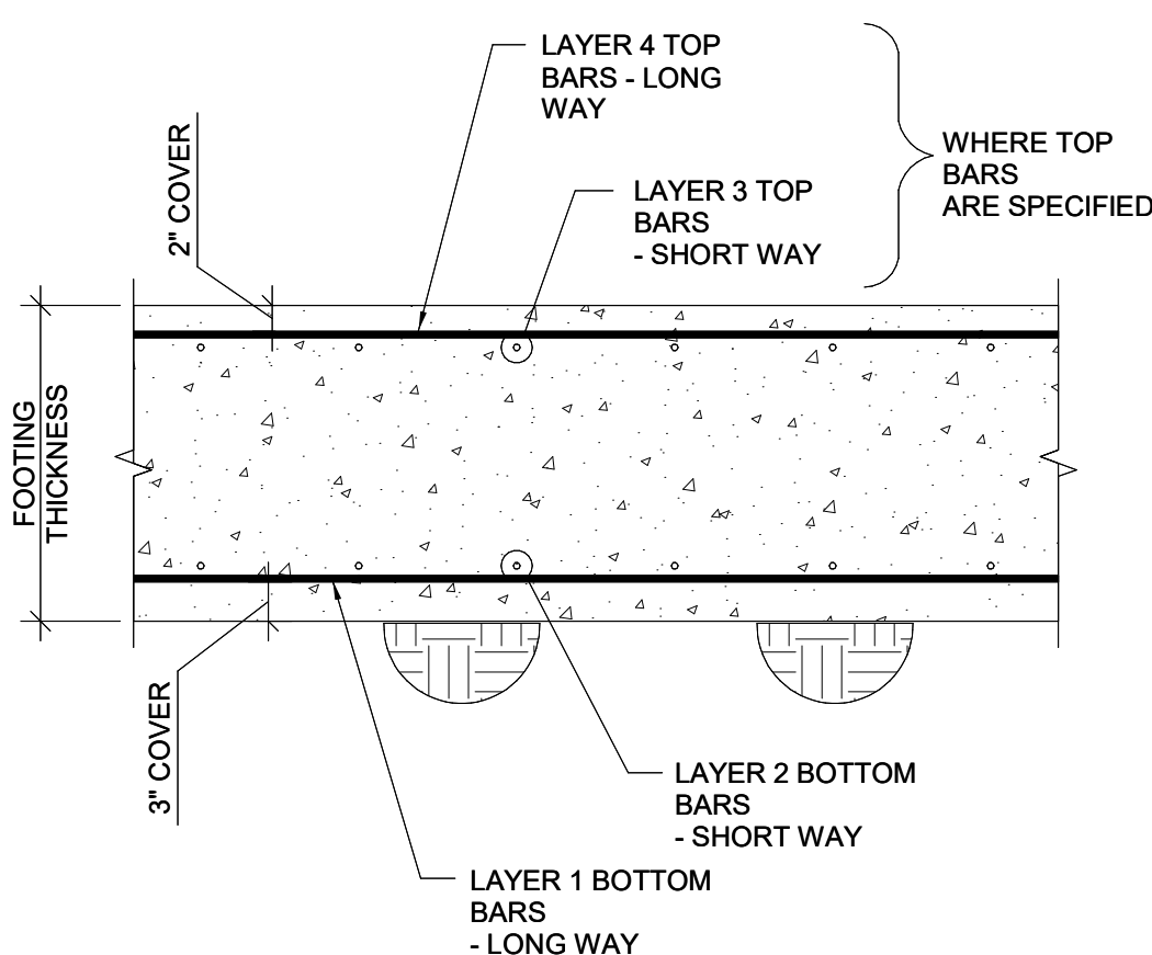
13 TYPICAL DETAIL BAR LAYER DIAGRAM RECTANGULAR SPREAD FOOTING 3/4" = 1'-0"
