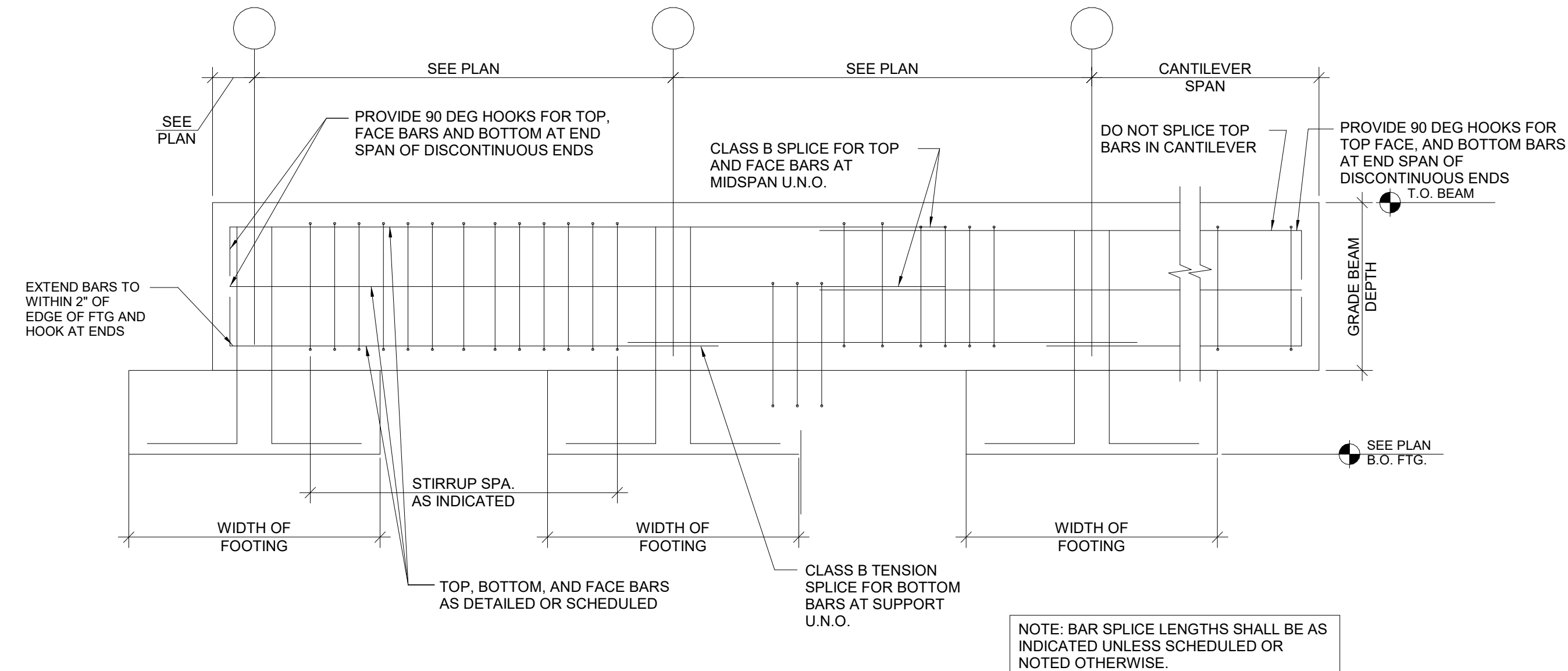
14 GRADE BEAM REINFORCING TYPICAL DETAIL 3/4" = 1'-0"
