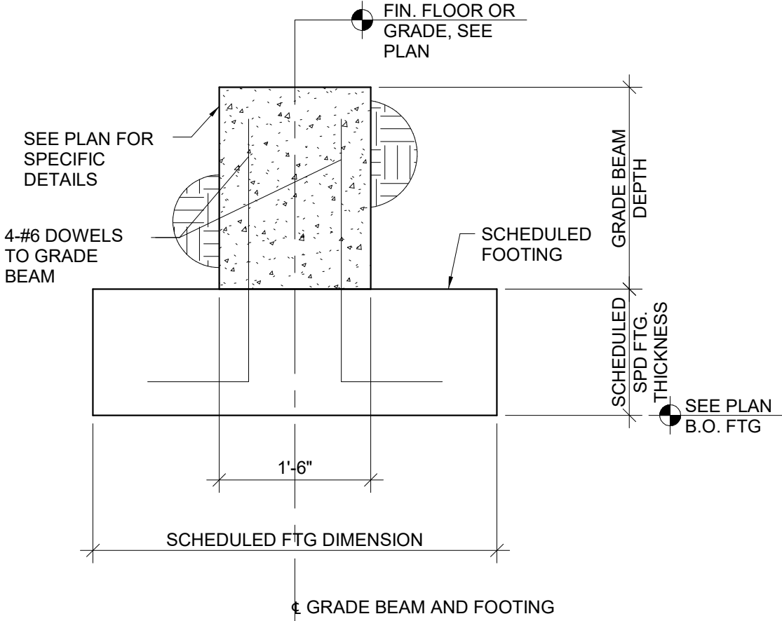
1 TYPICAL GRADE BEAM TO FOOTING DETAIL 3/4" = 1'-0"
