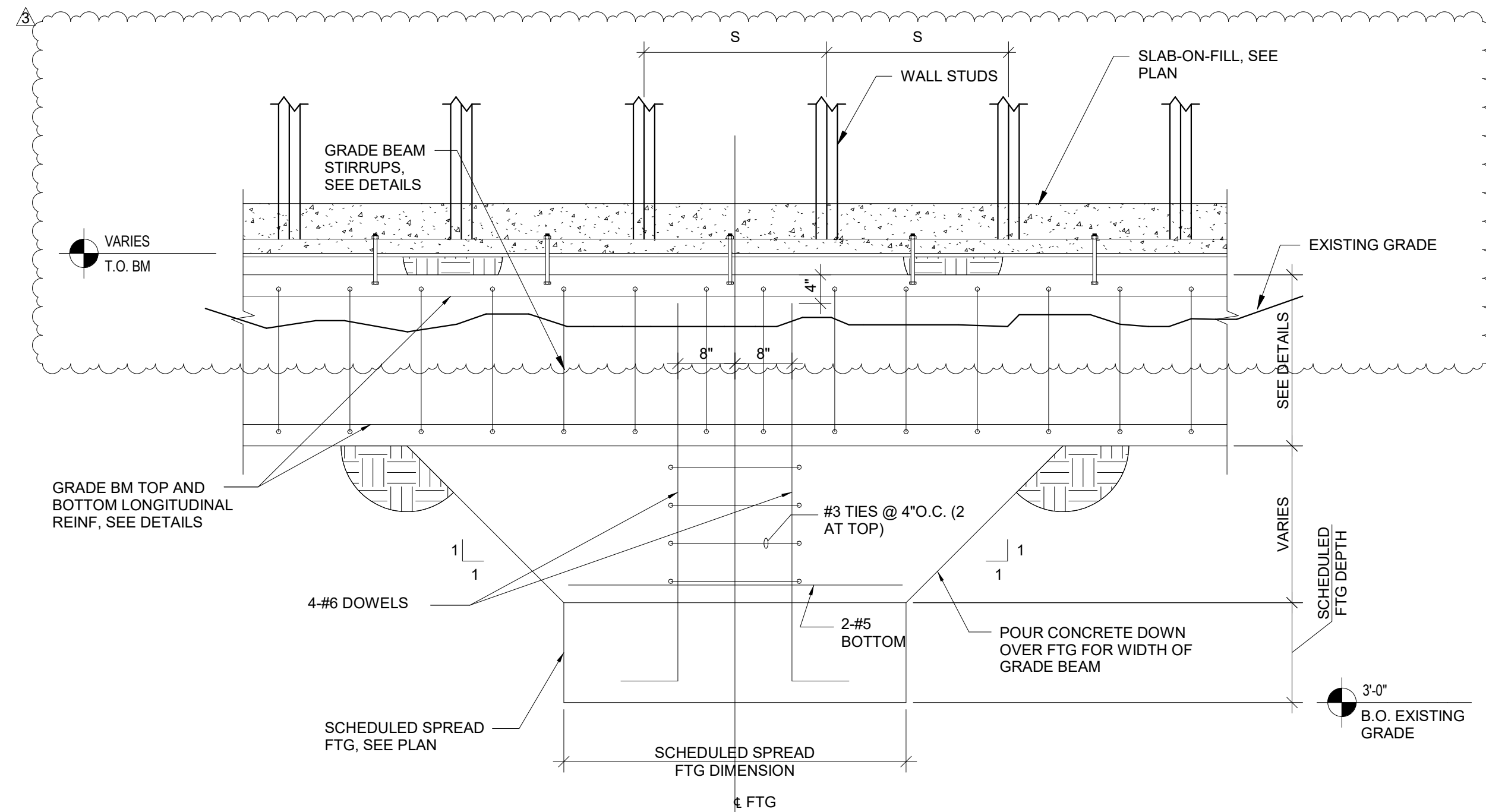
11 TYPICAL DETAIL FOOTING BEARING DEPTH GREATER THAN BOTTOM OF GRADE BEAM 3/4" = 1'-0"
