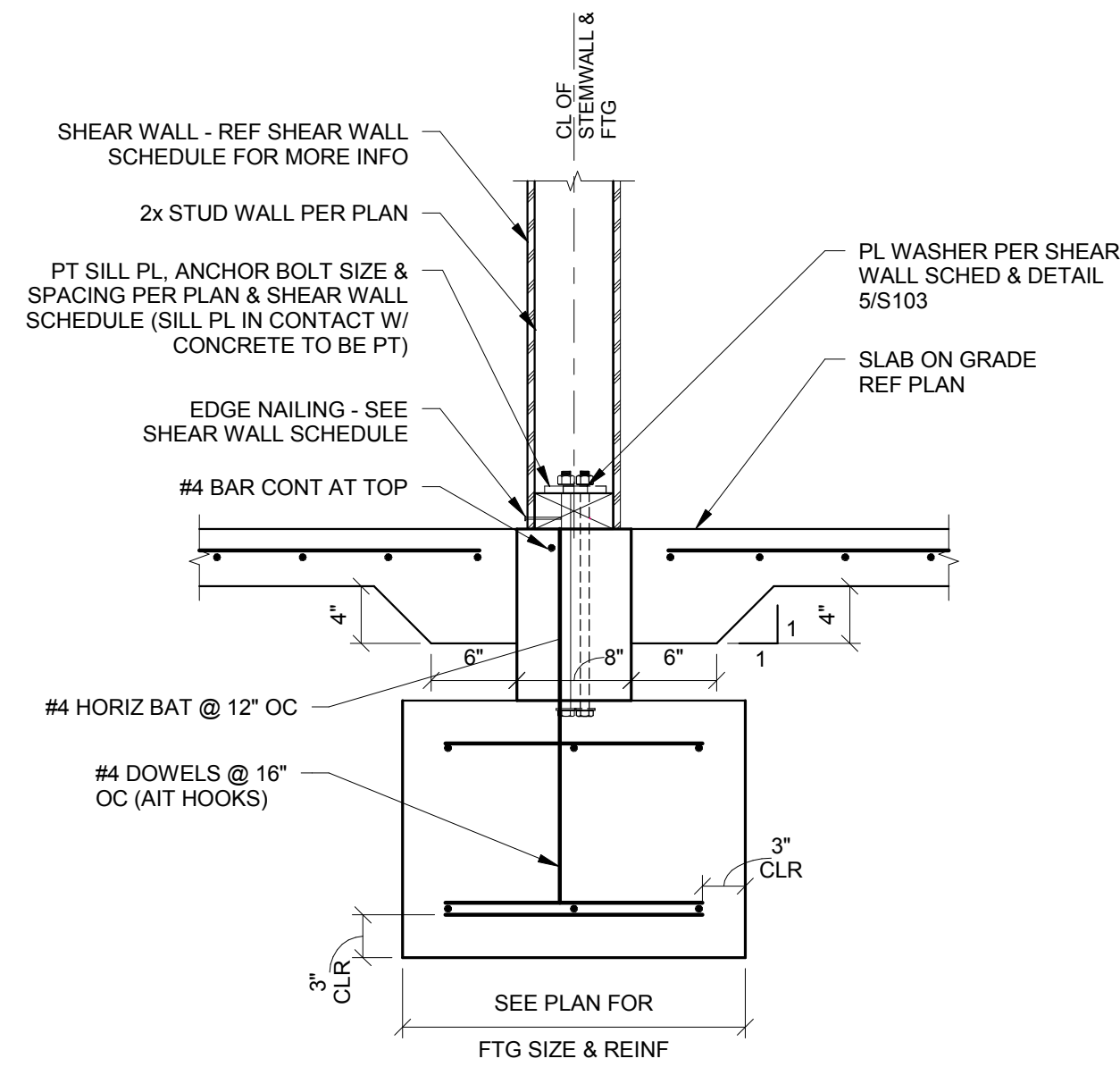
1 S500 INTERIOR SHEAR WALL TO THICKENED SLAB 1" = 1'-0"
