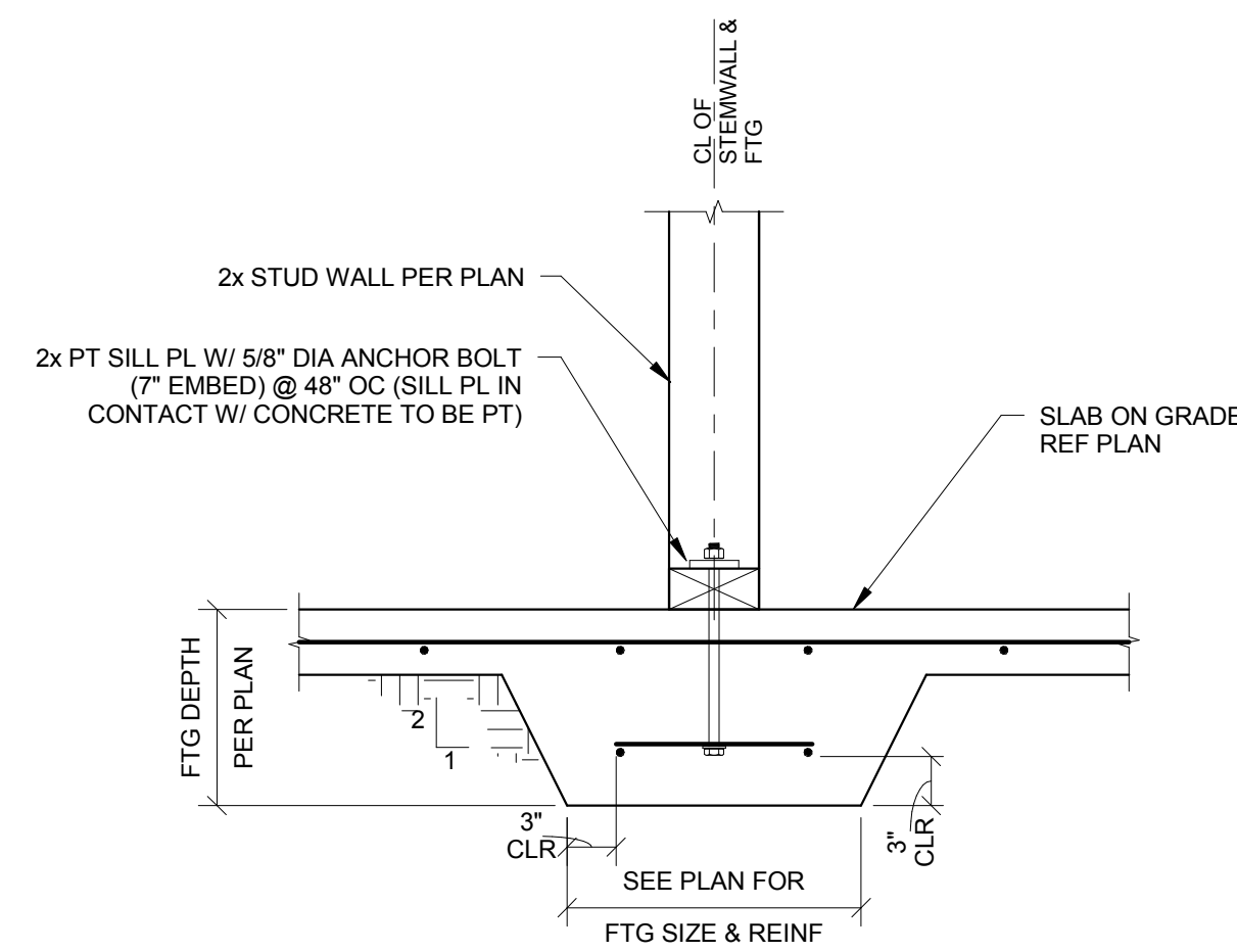
2 S500 INTERIOR SHEAR WALL TO THICKENED SLAB 1" = 1'-0"
