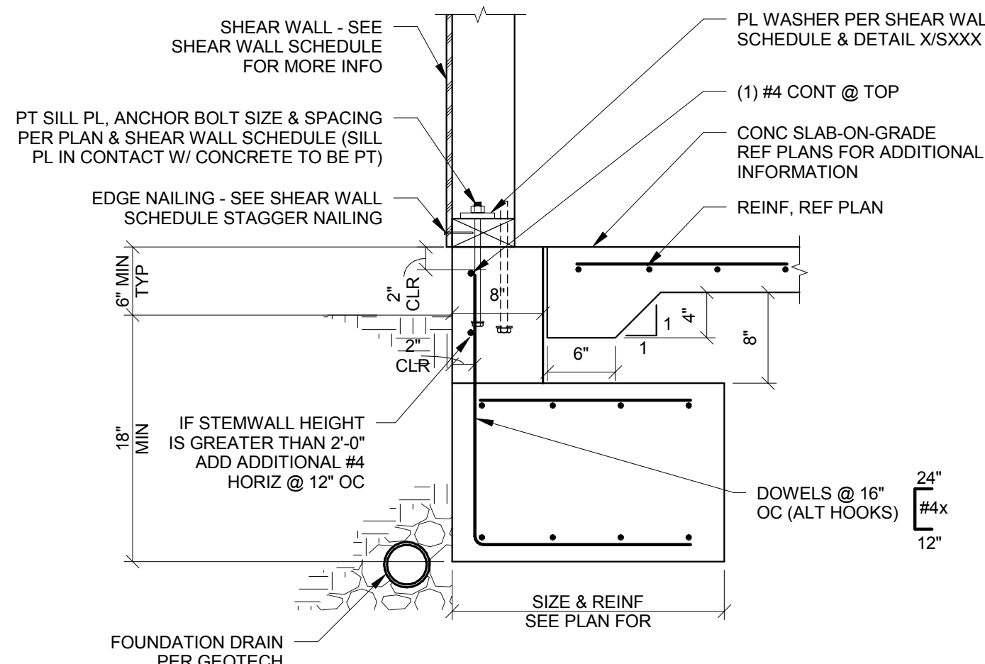
4 S500 EXTERIOR WALL AT FOUNDATION 1" = 1'-0"
