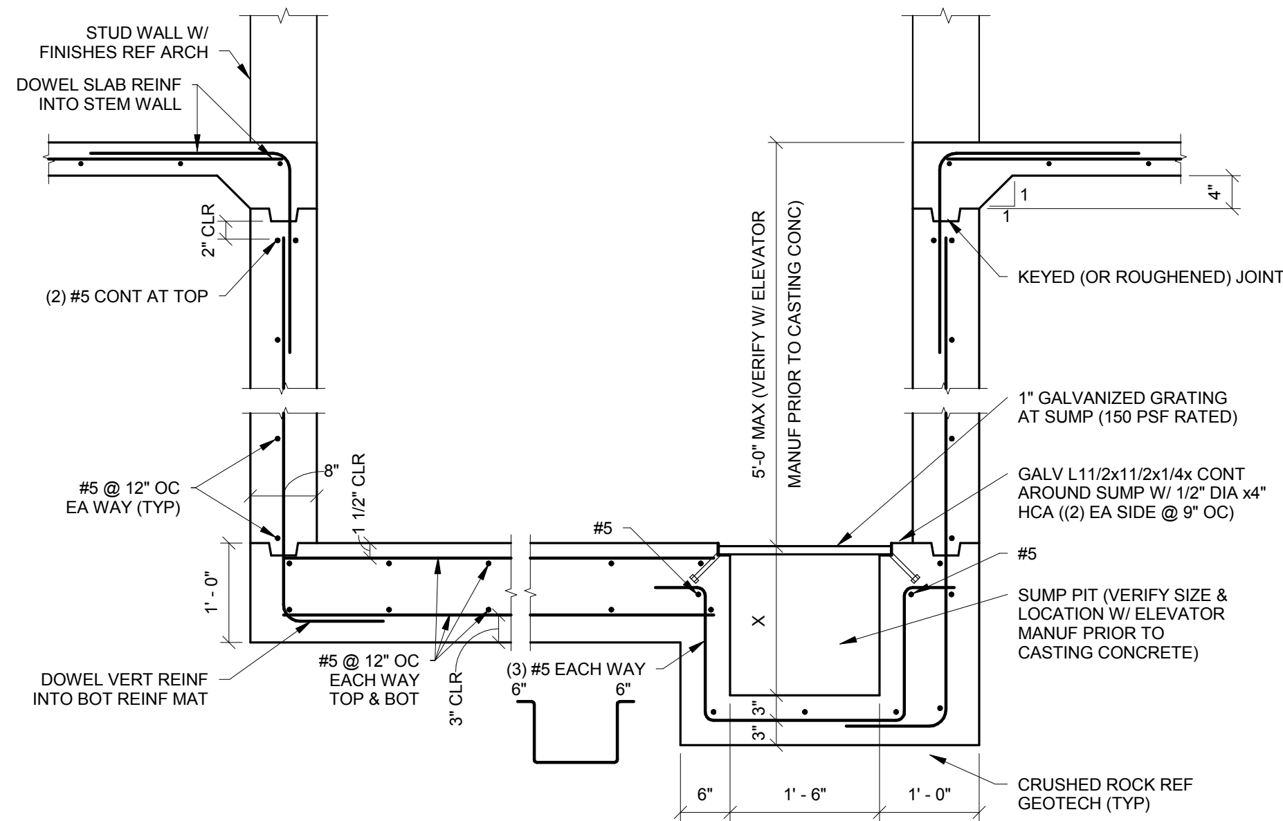
7 S500 ELEVATOR PIT - SECTION 3/4" = 1'-0"
