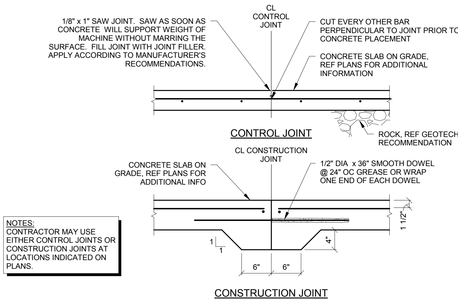
6 S500 SLAB JOINTS 1" = 1'-0"
