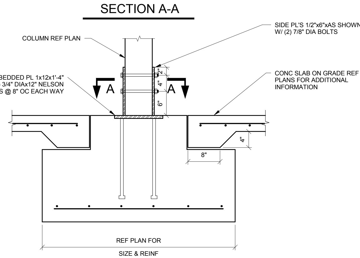
3 S500 GL COLUMN TO FOUNDATION 1" = 1'-0"
