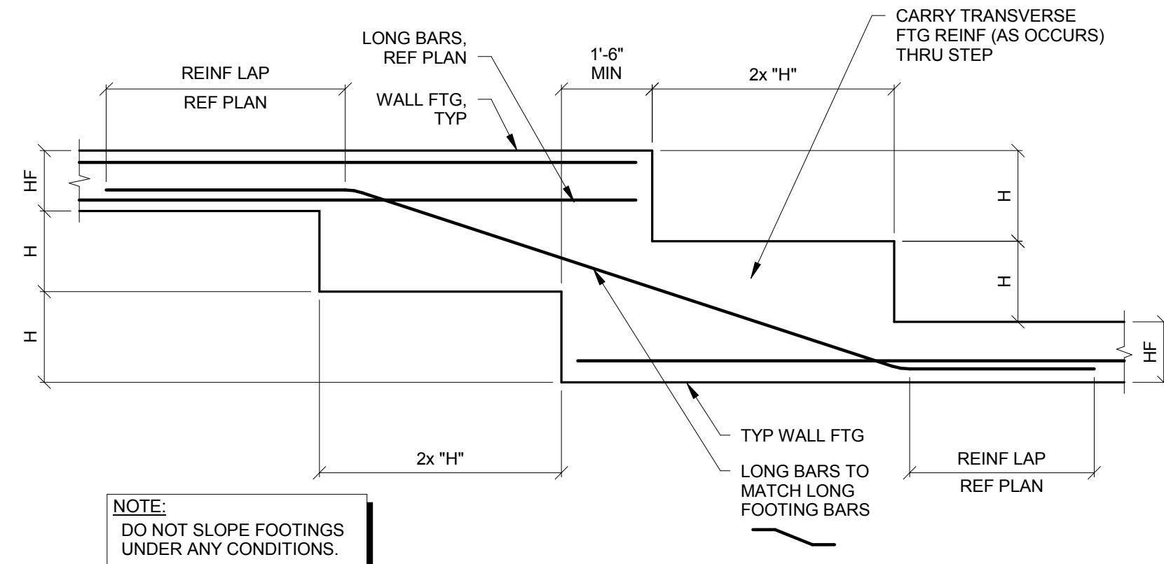
5 S500 STEPPED FOOTING 1" = 1'-0"
