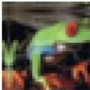
Augmented 1 frog
