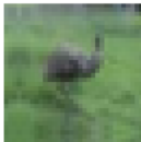
Augmented 4 bird
