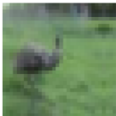
Augmented 1 bird
