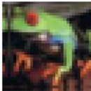
Augmented 2 frog
