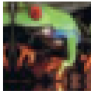
Augmented 3 frog
