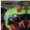
Augmented 4 frog
