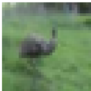
Original bird
