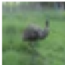
Augmented 3 bird
